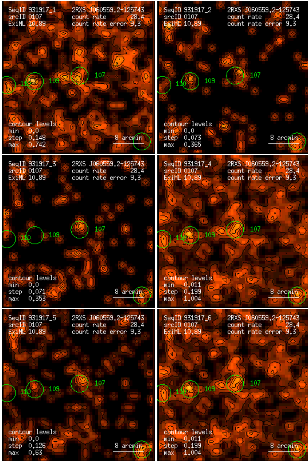
Figure 107: RASS 931917: detection 0107: band rate images, Gaussian filter: (1) PSPC channels 11 – 41, (2) 52 – 90, (3) 91 – 201, (4) 11 – 235, (5) 52 – 201, (6) 11 – 201. Broad band rates in counts/ks. Band rate contour levels in counts/ks/arcmin 2 .
