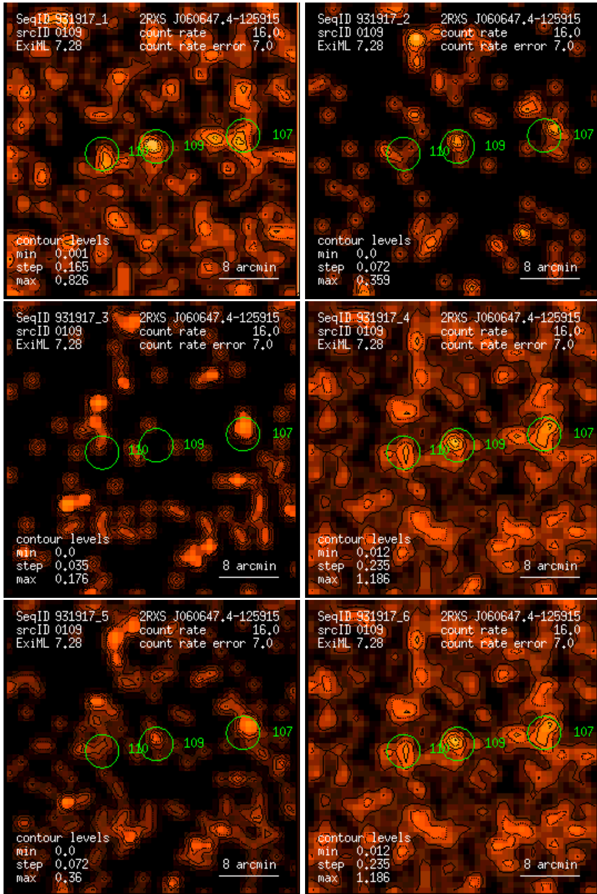
Figure 109: RASS 931917: detection 0109: band rate images, Gaussian filter: (1) PSPC channels 11 – 41, (2) 52 – 90, (3) 91 – 201, (4) 11 – 235, (5) 52 – 201, (6) 11 – 201. Broad band rates in counts/ks. Band rate contour levels in counts/ks/arcmin 2 .
