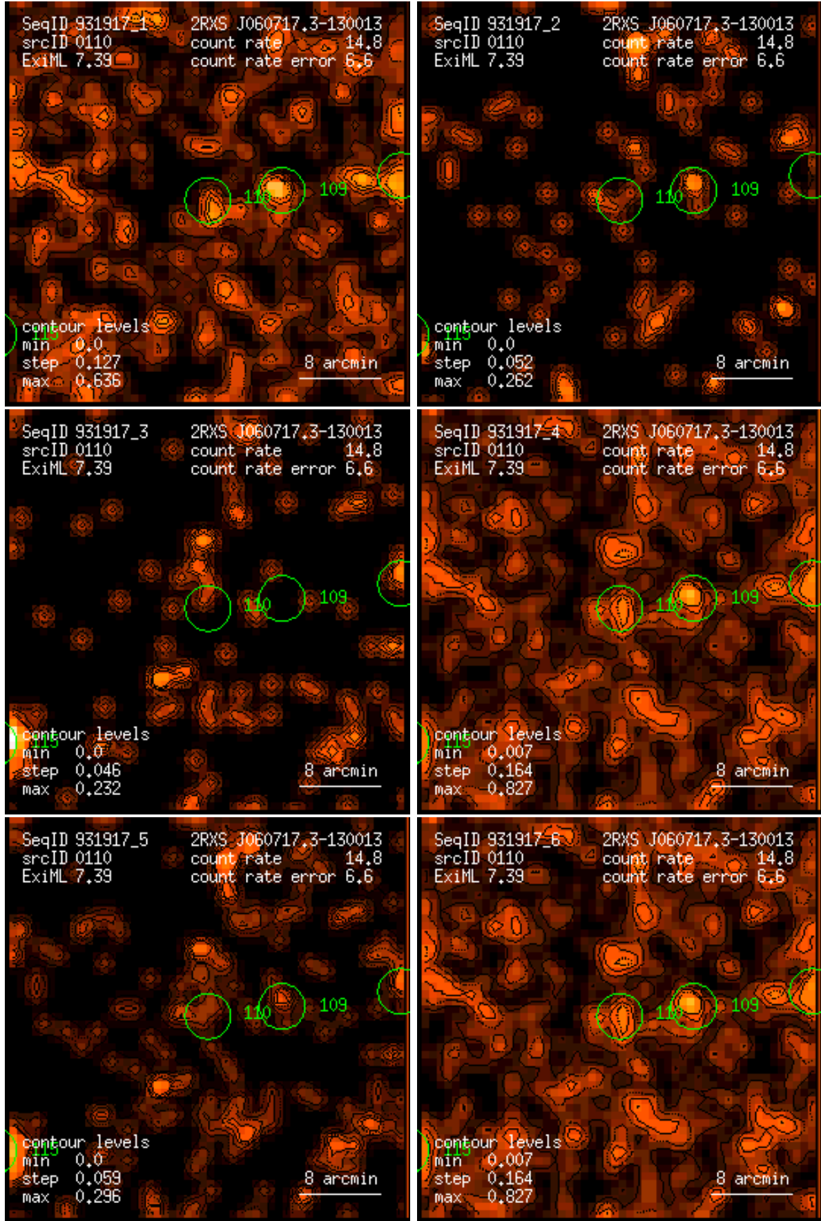
Figure 110: RASS 931917: detection 0110: band rate images, Gaussian filter: (1) PSPC channels 11 – 41, (2) 52 – 90, (3) 91 – 201, (4) 11 – 235, (5) 52 – 201, (6) 11 – 201. Broad band rates in counts/ks. Band rate contour levels in counts/ks/arcmin 2 .
