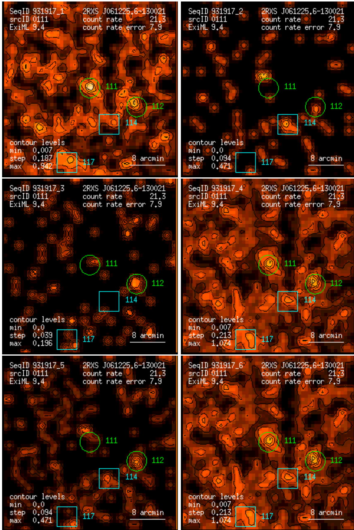
Figure 111: RASS 931917: detection 0111: band rate images, Gaussian filter: (1) PSPC channels 11 – 41, (2) 52 – 90, (3) 91 – 201, (4) 11 – 235, (5) 52 – 201, (6) 11 – 201. Broad band rates in counts/ks. Band rate contour levels in counts/ks/arcmin 2 .
