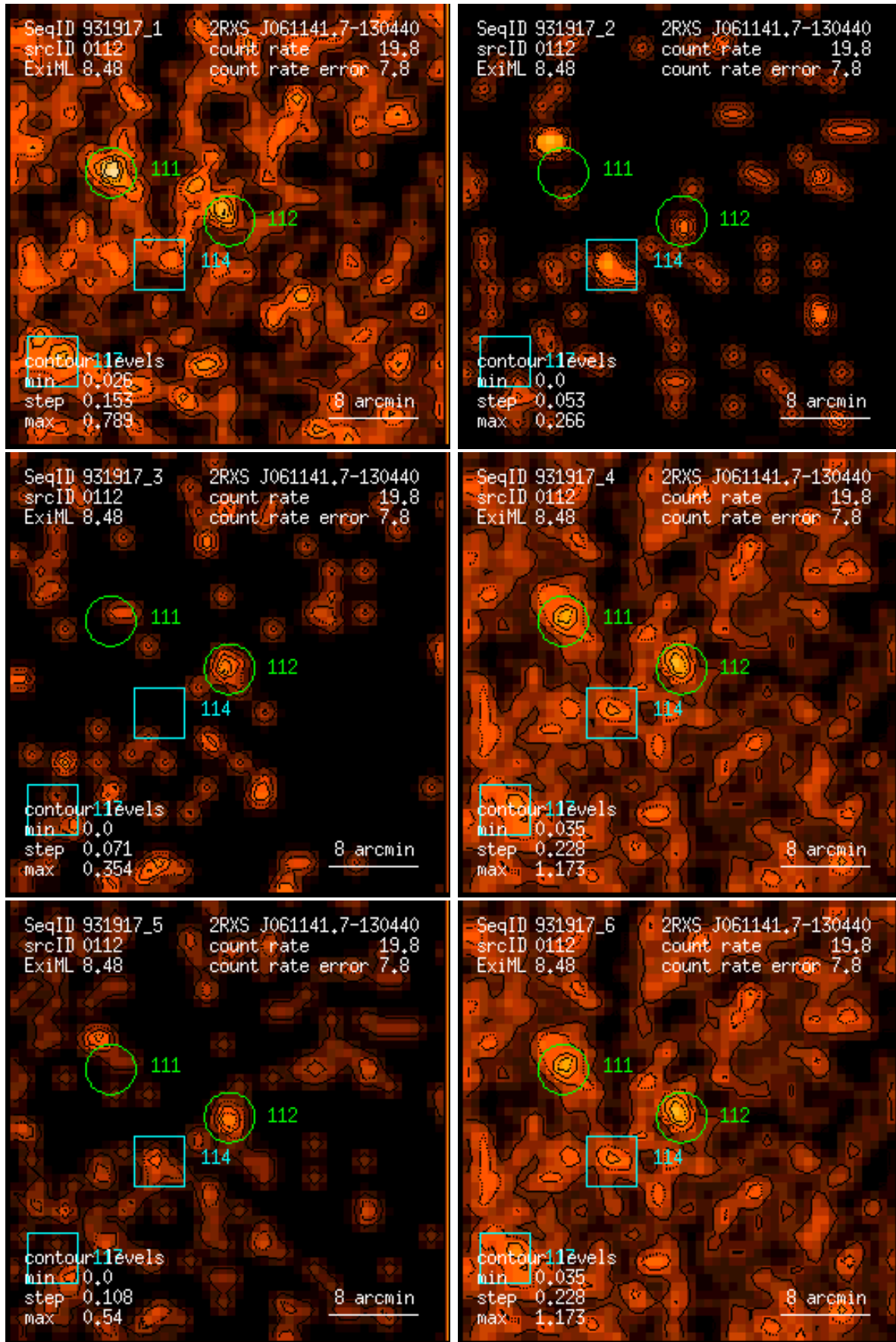
Figure 112: RASS 931917: detection 0112: band rate images, Gaussian filter: (1) PSPC channels 11 – 41, (2) 52 – 90, (3) 91 – 201, (4) 11 – 235, (5) 52 – 201, (6) 11 – 201. Broad band rates in counts/ks. Band rate contour levels in counts/ks/arcmin 2 .
