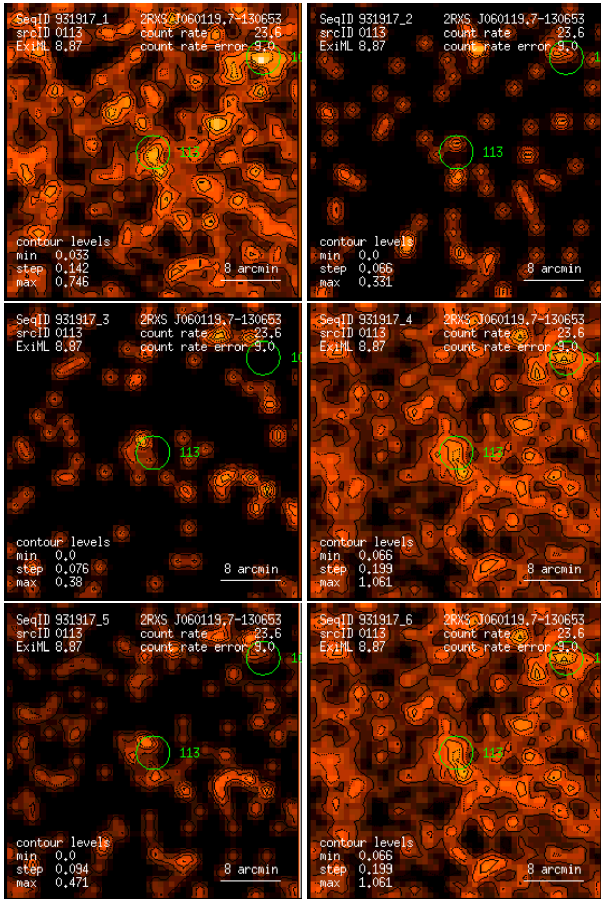
Figure 113: RASS 931917: detection 0113: band rate images, Gaussian filter: (1) PSPC channels 11 – 41, (2) 52 – 90, (3) 91 – 201, (4) 11 – 235, (5) 52 – 201, (6) 11 – 201. Broad band rates in counts/ks. Band rate contour levels in counts/ks/arcmin 2 .
