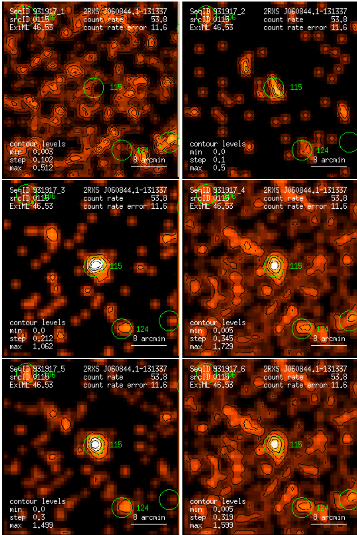
Figure 115: RASS 931917: detection 0115: band rate images, Gaussian filter: (1) PSPC channels 11 – 41, (2) 52 – 90, (3) 91 – 201, (4) 11 – 235, (5) 52 – 201, (6) 11 – 201. Broad band rates in counts/ks. Band rate contour levels in counts/ks/arcmin 2 .
