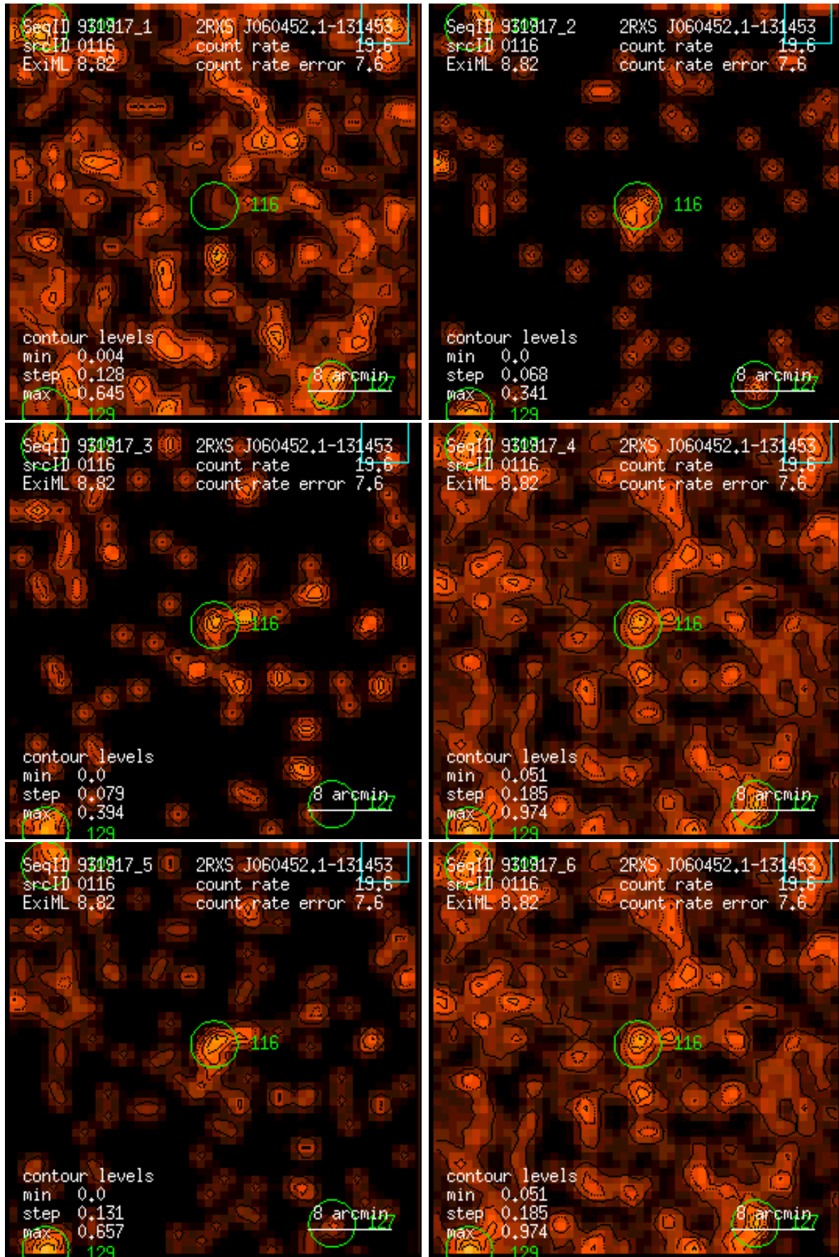
Figure 116: RASS 931917: detection 0116: band rate images, Gaussian filter: (1) PSPC channels 11 – 41, (2) 52 – 90, (3) 91 – 201, (4) 11 – 235, (5) 52 – 201, (6) 11 – 201. Broad band rates in counts/ks. Band rate contour levels in counts/ks/arcmin 2 .
