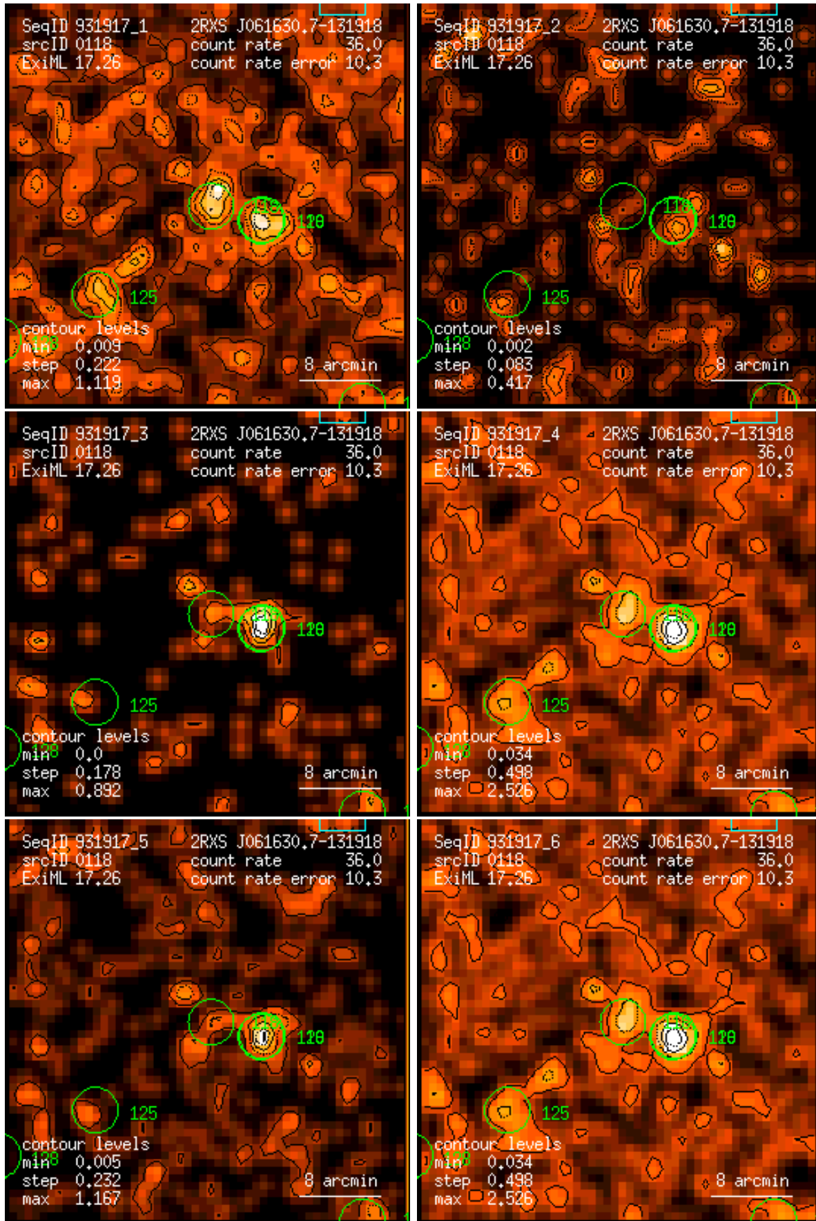
Figure 118: RASS 931917: detection 0118: band rate images, Gaussian filter: (1) PSPC channels 11 – 41, (2) 52 – 90, (3) 91 – 201, (4) 11 – 235, (5) 52 – 201, (6) 11 – 201. Broad band rates in counts/ks. Band rate contour levels in counts/ks/arcmin 2 .
