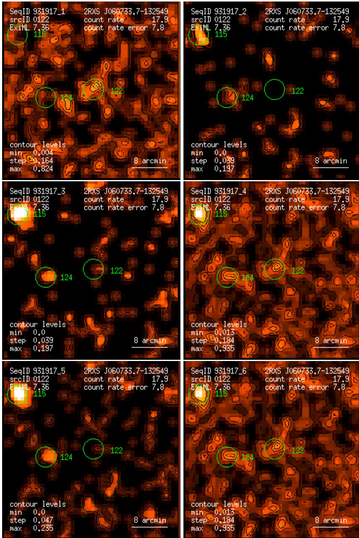
Figure 122: RASS 931917: detection 0122: band rate images, Gaussian filter: (1) PSPC channels 11 – 41, (2) 52 – 90, (3) 91 – 201, (4) 11 – 235, (5) 52 – 201, (6) 11 – 201. Broad band rates in counts/ks. Band rate contour levels in counts/ks/arcmin 2 .
