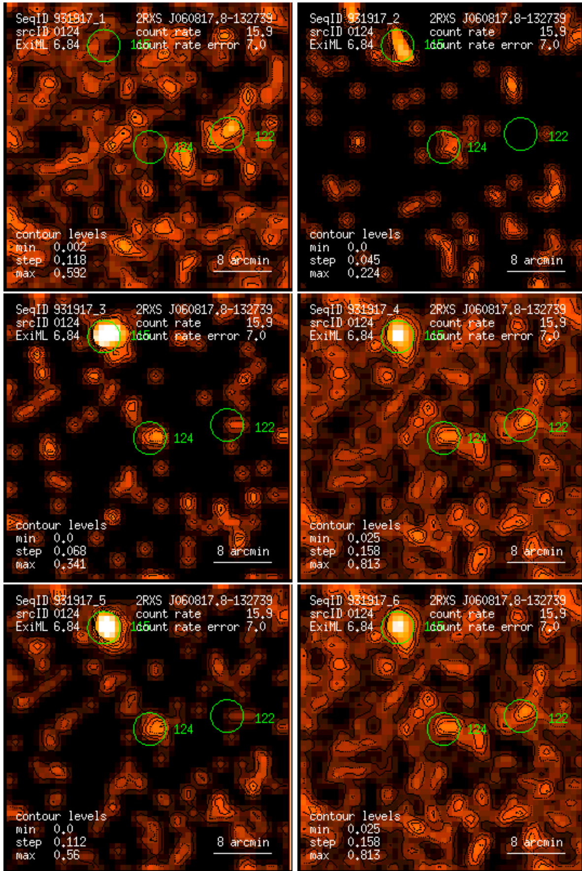
Figure 124: RASS 931917: detection 0124: band rate images, Gaussian filter: (1) PSPC channels 11 – 41, (2) 52 – 90, (3) 91 – 201, (4) 11 – 235, (5) 52 – 201, (6) 11 – 201. Broad band rates in counts/ks. Band rate contour levels in counts/ks/arcmin 2 .
