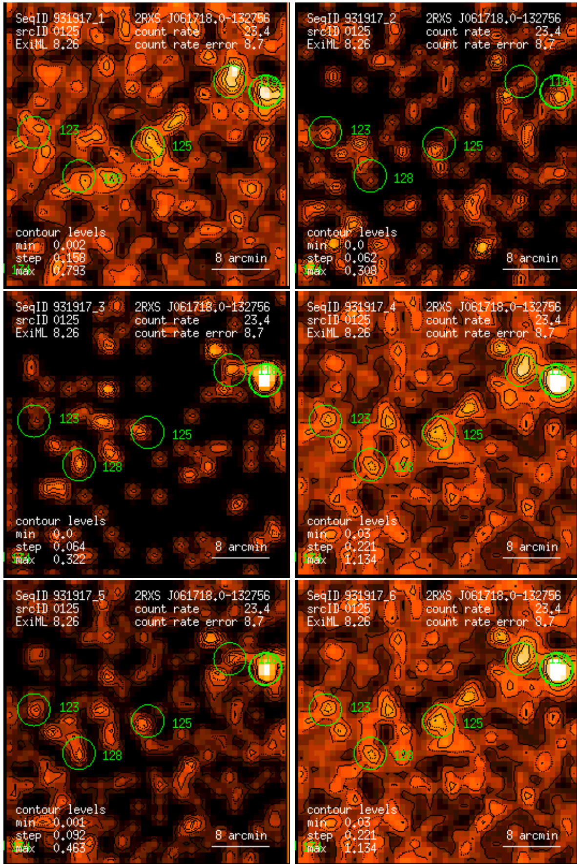
Figure 125: RASS 931917: detection 0125: band rate images, Gaussian filter: (1) PSPC channels 11 – 41, (2) 52 – 90, (3) 91 – 201, (4) 11 – 235, (5) 52 – 201, (6) 11 – 201. Broad band rates in counts/ks. Band rate contour levels in counts/ks/arcmin 2 .
