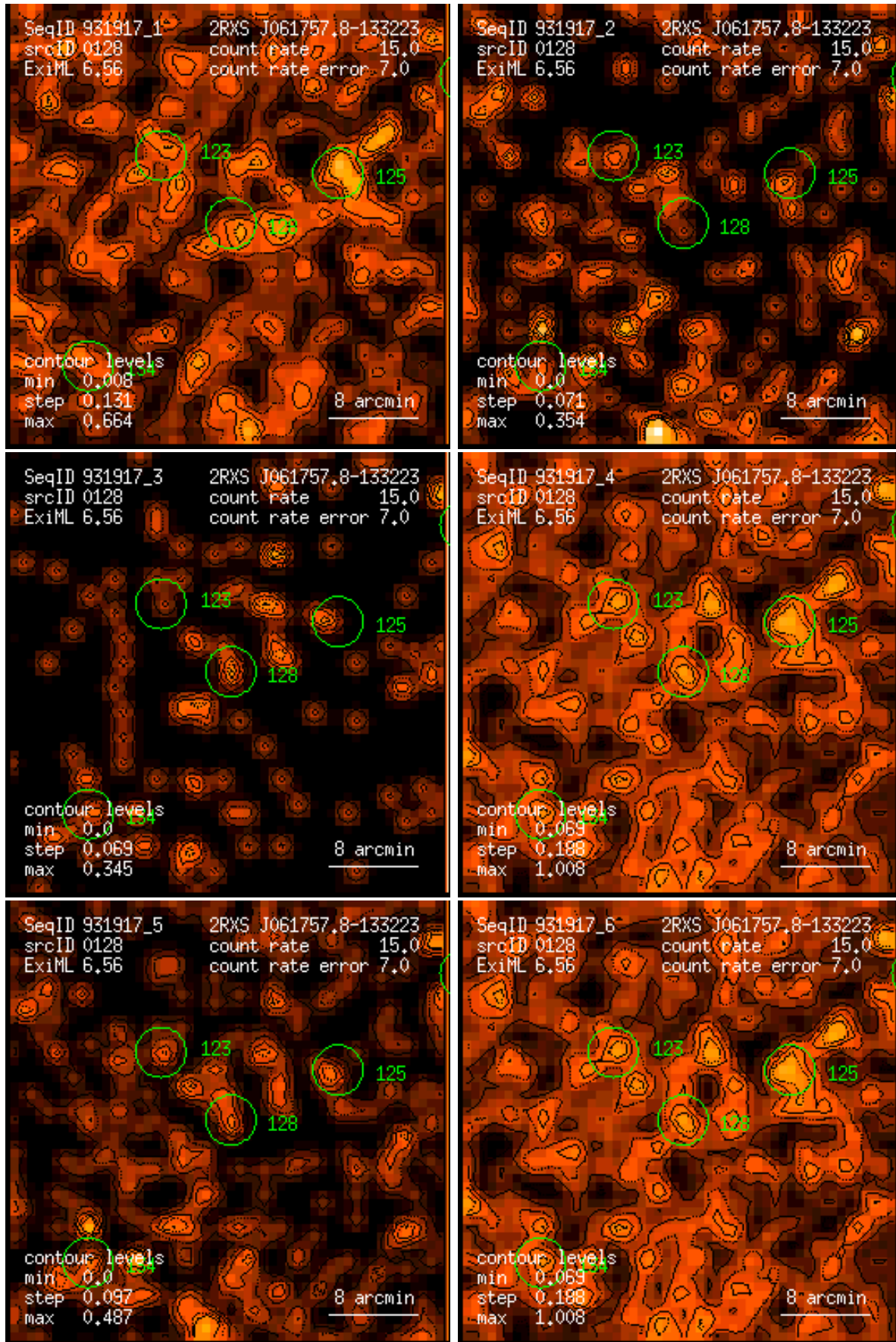
Figure 128: RASS 931917: detection 0128: band rate images, Gaussian filter: (1) PSPC channels 11 – 41, (2) 52 – 90, (3) 91 – 201, (4) 11 – 235, (5) 52 – 201, (6) 11 – 201. Broad band rates in counts/ks. Band rate contour levels in counts/ks/arcmin 2 .
