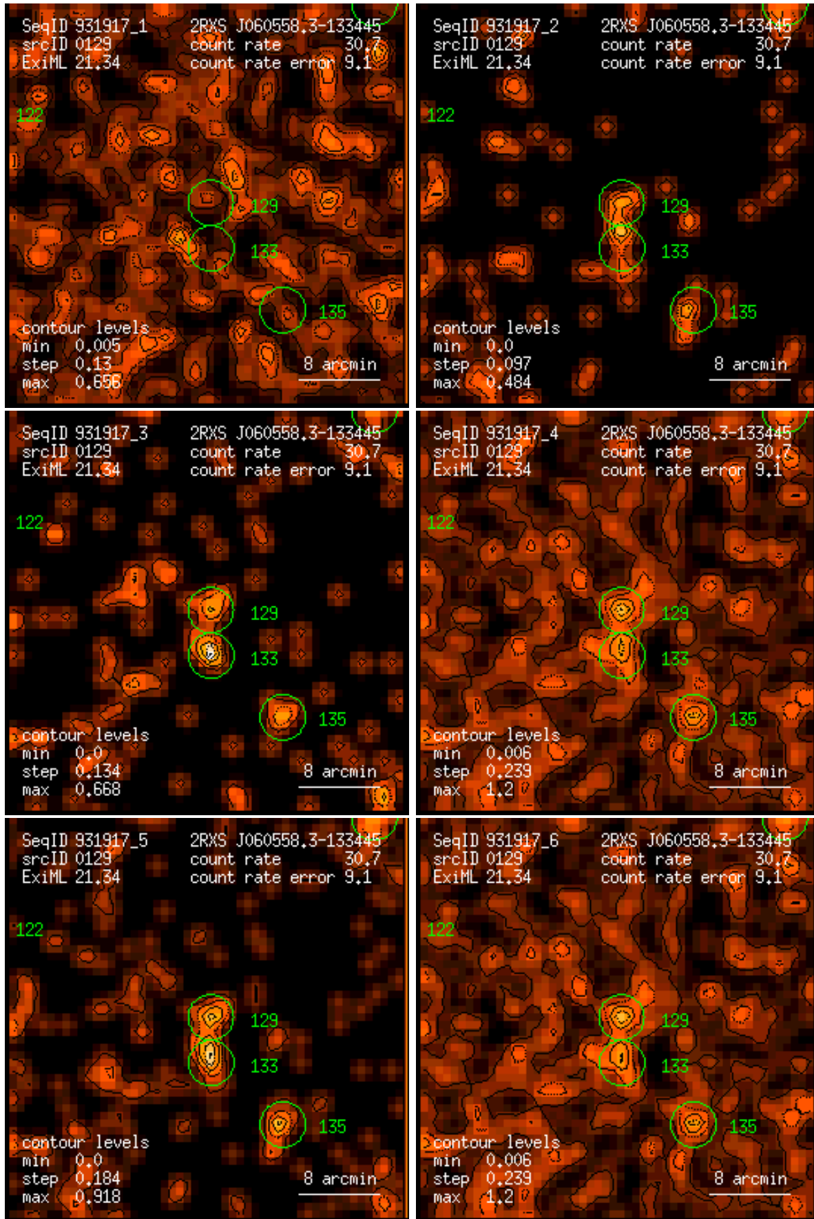
Figure 129: RASS 931917: detection 0129: band rate images, Gaussian filter: (1) PSPC channels 11 – 41, (2) 52 – 90, (3) 91 – 201, (4) 11 – 235, (5) 52 – 201, (6) 11 – 201. Broad band rates in counts/ks. Band rate contour levels in counts/ks/arcmin 2 .
