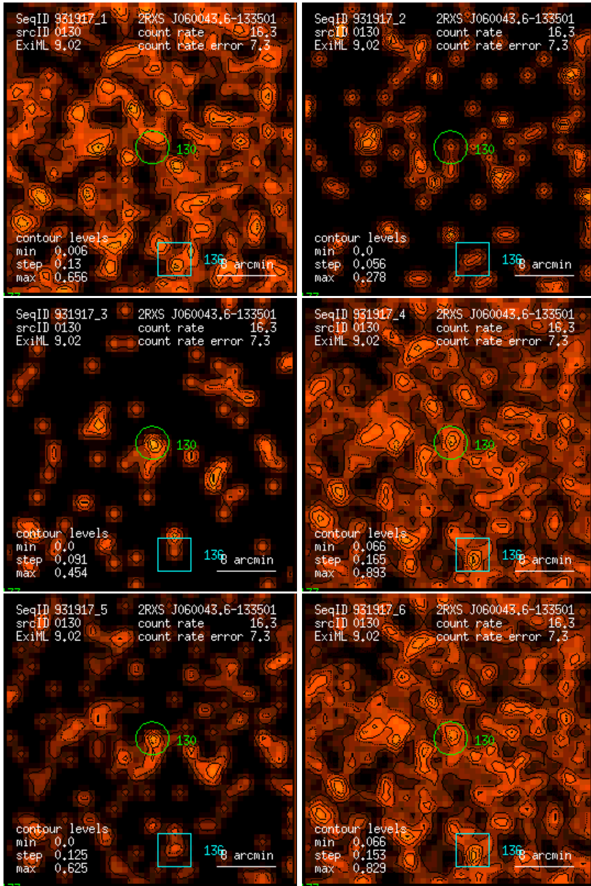
Figure 130: RASS 931917: detection 0130: band rate images, Gaussian filter: (1) PSPC channels 11 – 41, (2) 52 – 90, (3) 91 – 201, (4) 11 – 235, (5) 52 – 201, (6) 11 – 201. Broad band rates in counts/ks. Band rate contour levels in counts/ks/arcmin 2 .
