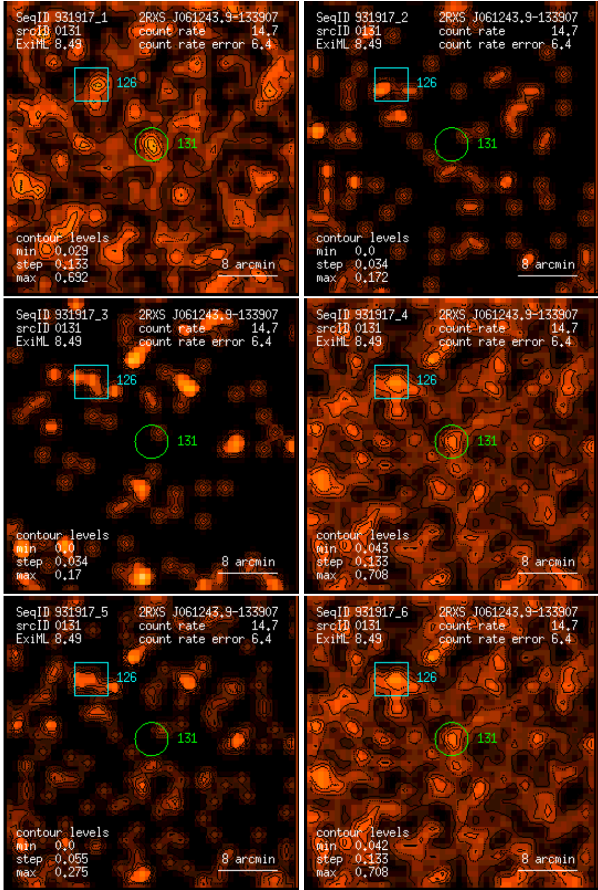
Figure 131: RASS 931917: detection 0131: band rate images, Gaussian filter: (1) PSPC channels 11 – 41, (2) 52 – 90, (3) 91 – 201, (4) 11 – 235, (5) 52 – 201, (6) 11 – 201. Broad band rates in counts/ks. Band rate contour levels in counts/ks/arcmin 2 .
