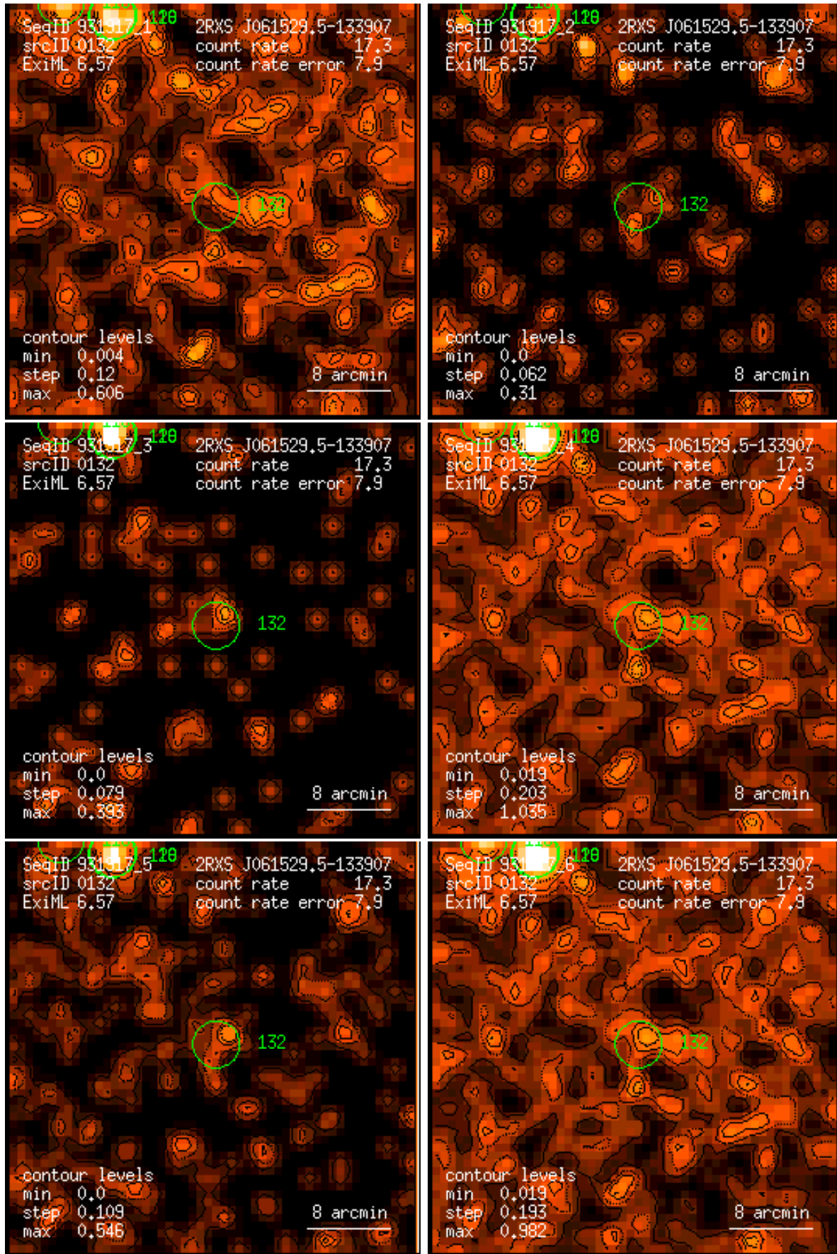
Figure 132: RASS 931917: detection 0132: band rate images, Gaussian filter: (1) PSPC channels 11 – 41, (2) 52 – 90, (3) 91 – 201, (4) 11 – 235, (5) 52 – 201, (6) 11 – 201. Broad band rates in counts/ks. Band rate contour levels in counts/ks/arcmin 2 .
