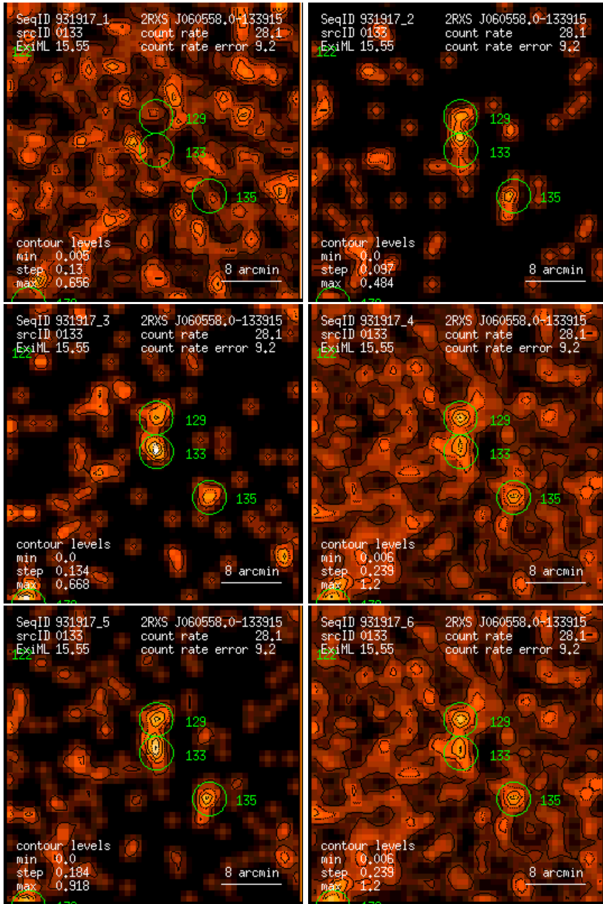
Figure 133: RASS 931917: detection 0133: band rate images, Gaussian filter: (1) PSPC channels 11 – 41, (2) 52 – 90, (3) 91 – 201, (4) 11 – 235, (5) 52 – 201, (6) 11 – 201. Broad band rates in counts/ks. Band rate contour levels in counts/ks/arcmin 2 .
