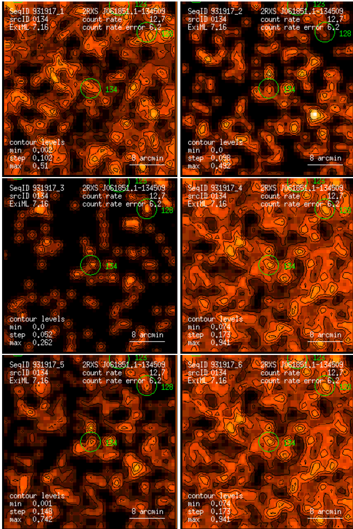
Figure 134: RASS 931917: detection 0134: band rate images, Gaussian filter: (1) PSPC channels 11 – 41, (2) 52 – 90, (3) 91 – 201, (4) 11 – 235, (5) 52 – 201, (6) 11 – 201. Broad band rates in counts/ks. Band rate contour levels in counts/ks/arcmin 2 .
