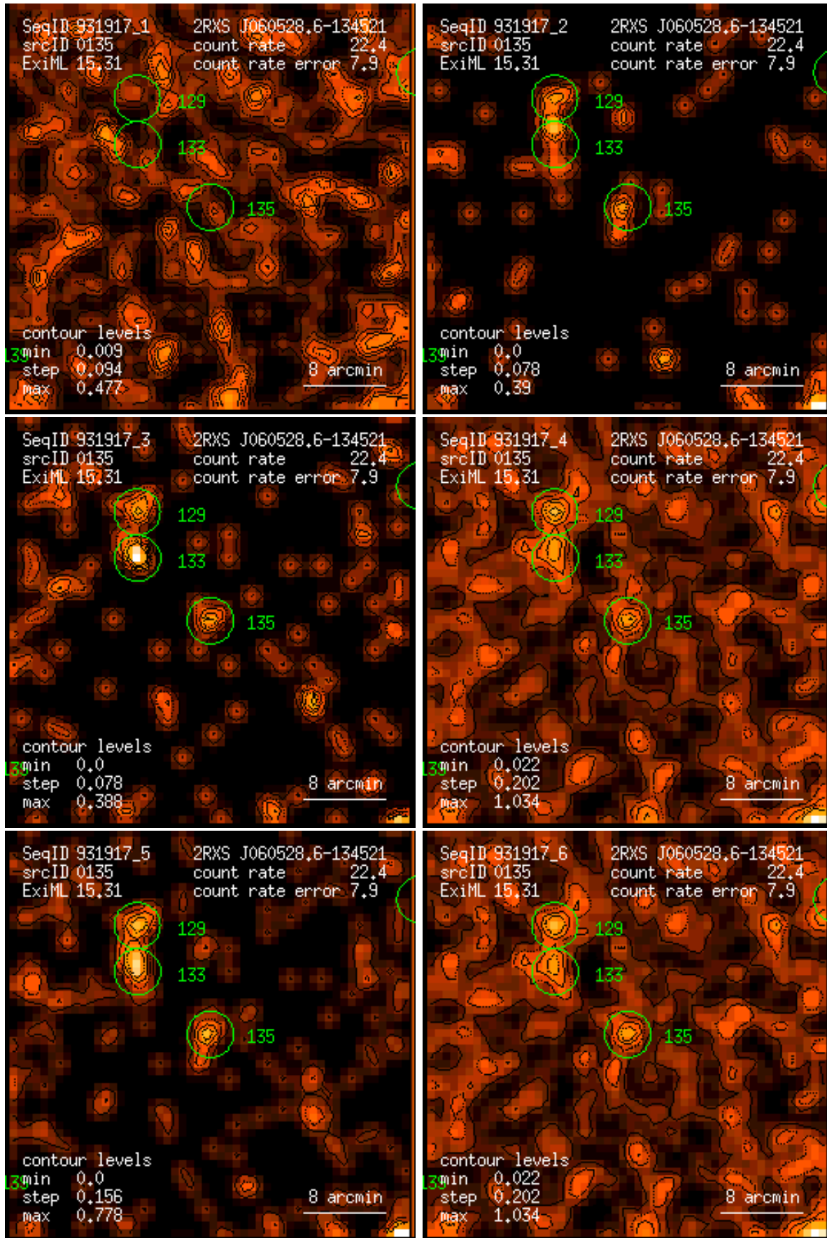
Figure 135: RASS 931917: detection 0135: band rate images, Gaussian filter: (1) PSPC channels 11 – 41, (2) 52 – 90, (3) 91 – 201, (4) 11 – 235, (5) 52 – 201, (6) 11 – 201. Broad band rates in counts/ks. Band rate contour levels in counts/ks/arcmin 2 .
