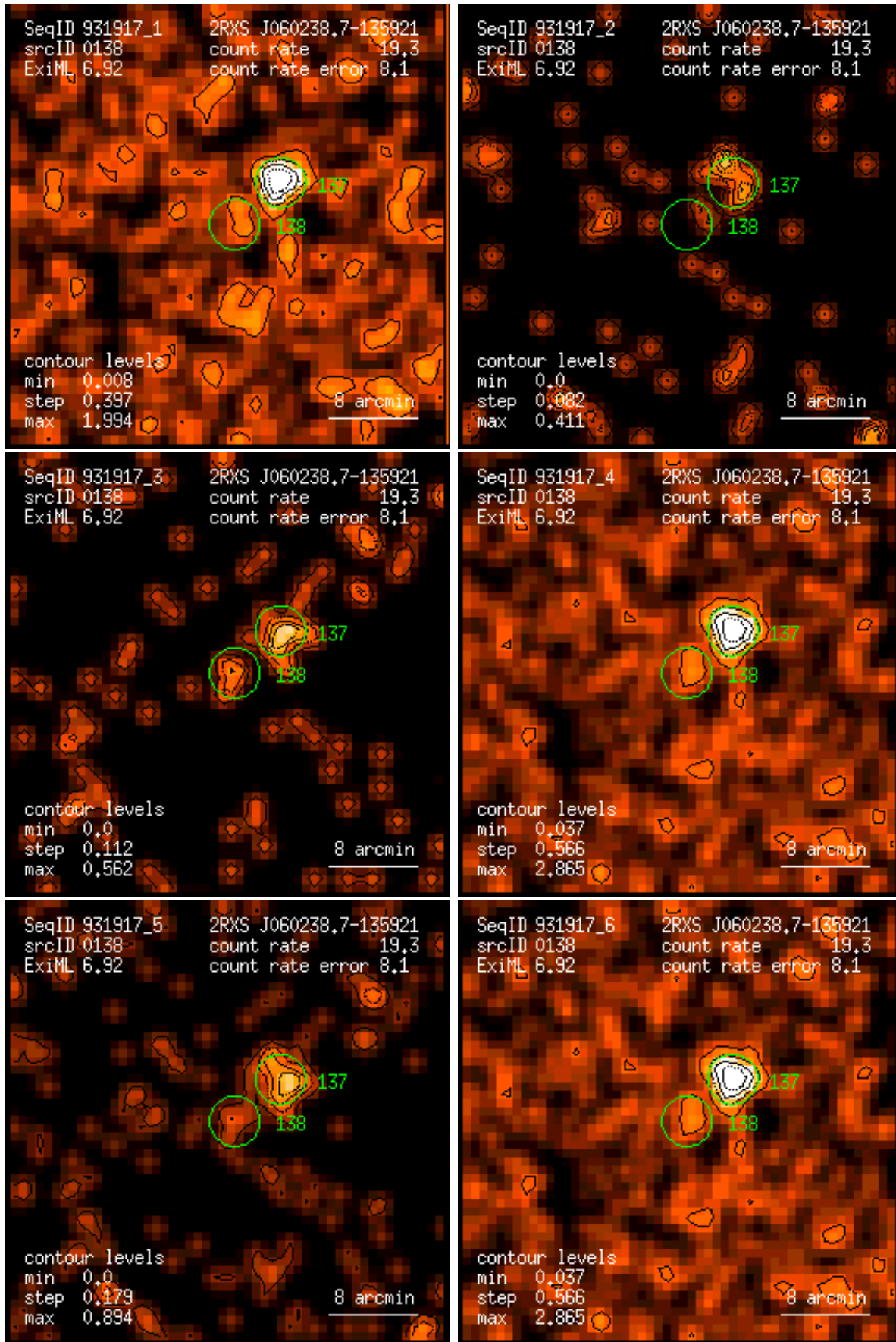
Figure 138: RASS 931917: detection 0138: band rate images, Gaussian filter: (1) PSPC channels 11 – 41, (2) 52 – 90, (3) 91 – 201, (4) 11 – 235, (5) 52 – 201, (6) 11 – 201. Broad band rates in counts/ks. Band rate contour levels in counts/ks/arcmin 2 .
