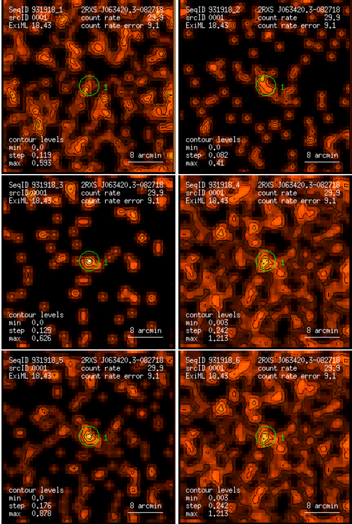
Figure 1: RASS 931918: detection 0001: band rate images, Gaussian filter: (1) PSPC channels 11 – 41, (2) 52 – 90, (3) 91 – 201, (4) 11 – 235, (5) 52 – 201, (6) 11 – 201. Broad band rates in counts/ks. Band rate contour levels in counts/ks/arcmin 2 .
