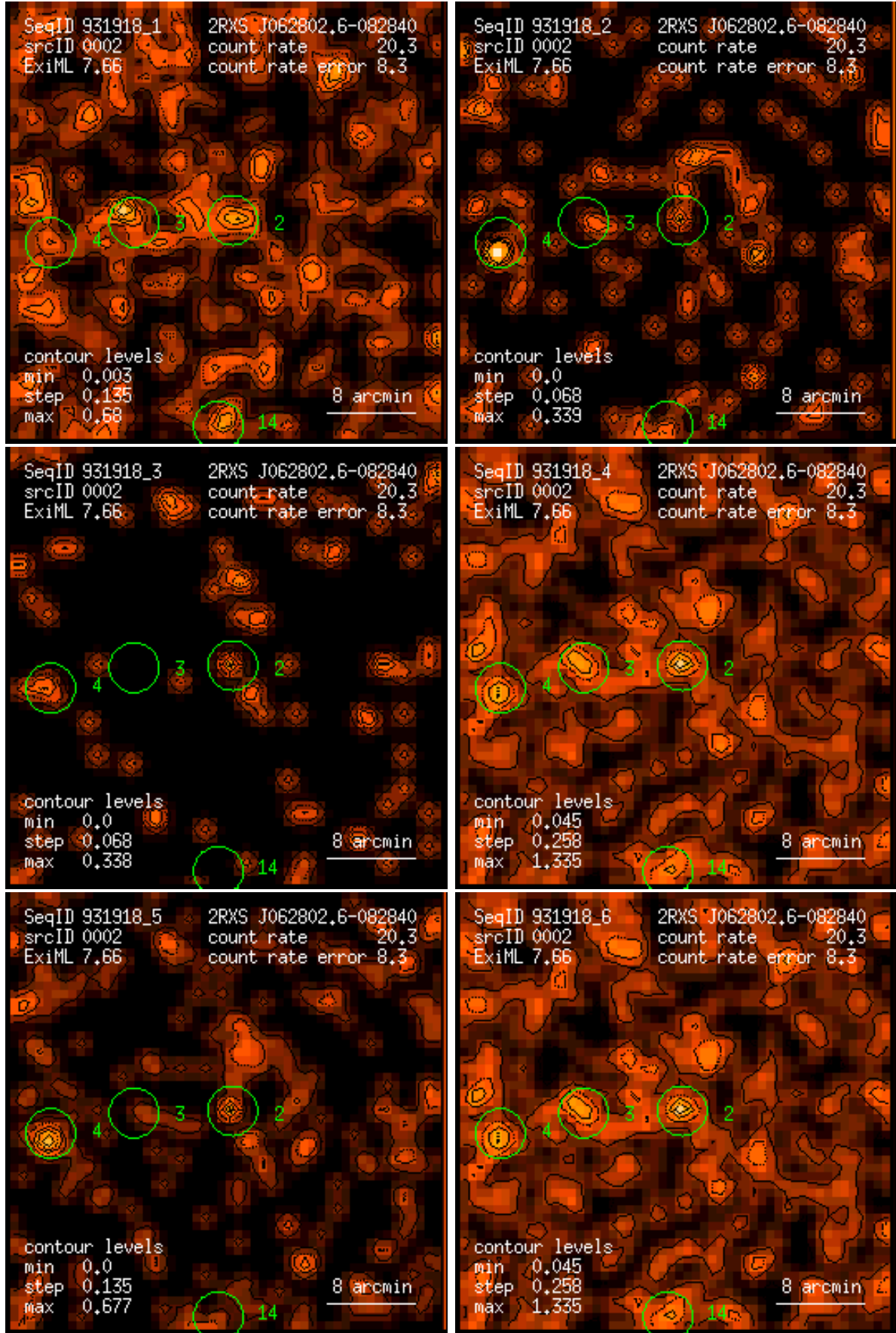
Figure 2: RASS 931918: detection 0002: band rate images, Gaussian filter: (1) PSPC channels 11 – 41, (2) 52 – 90, (3) 91 – 201, (4) 11 – 235, (5) 52 – 201, (6) 11 – 201. Broad band rates in counts/ks. Band rate contour levels in counts/ks/arcmin 2 .
