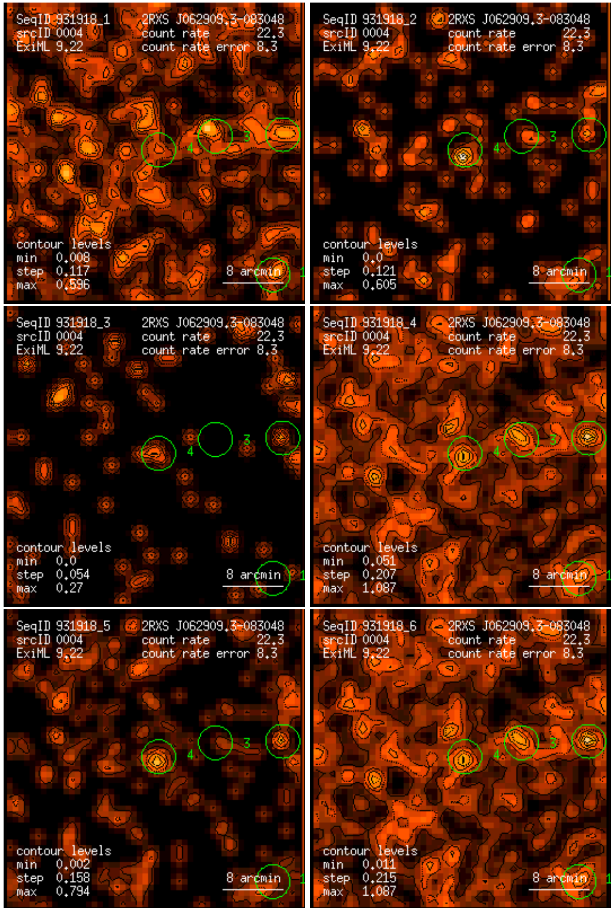
Figure 4: RASS 931918: detection 0004: band rate images, Gaussian filter: (1) PSPC channels 11 – 41, (2) 52 – 90, (3) 91 – 201, (4) 11 – 235, (5) 52 – 201, (6) 11 – 201. Broad band rates in counts/ks. Band rate contour levels in counts/ks/arcmin 2 .
