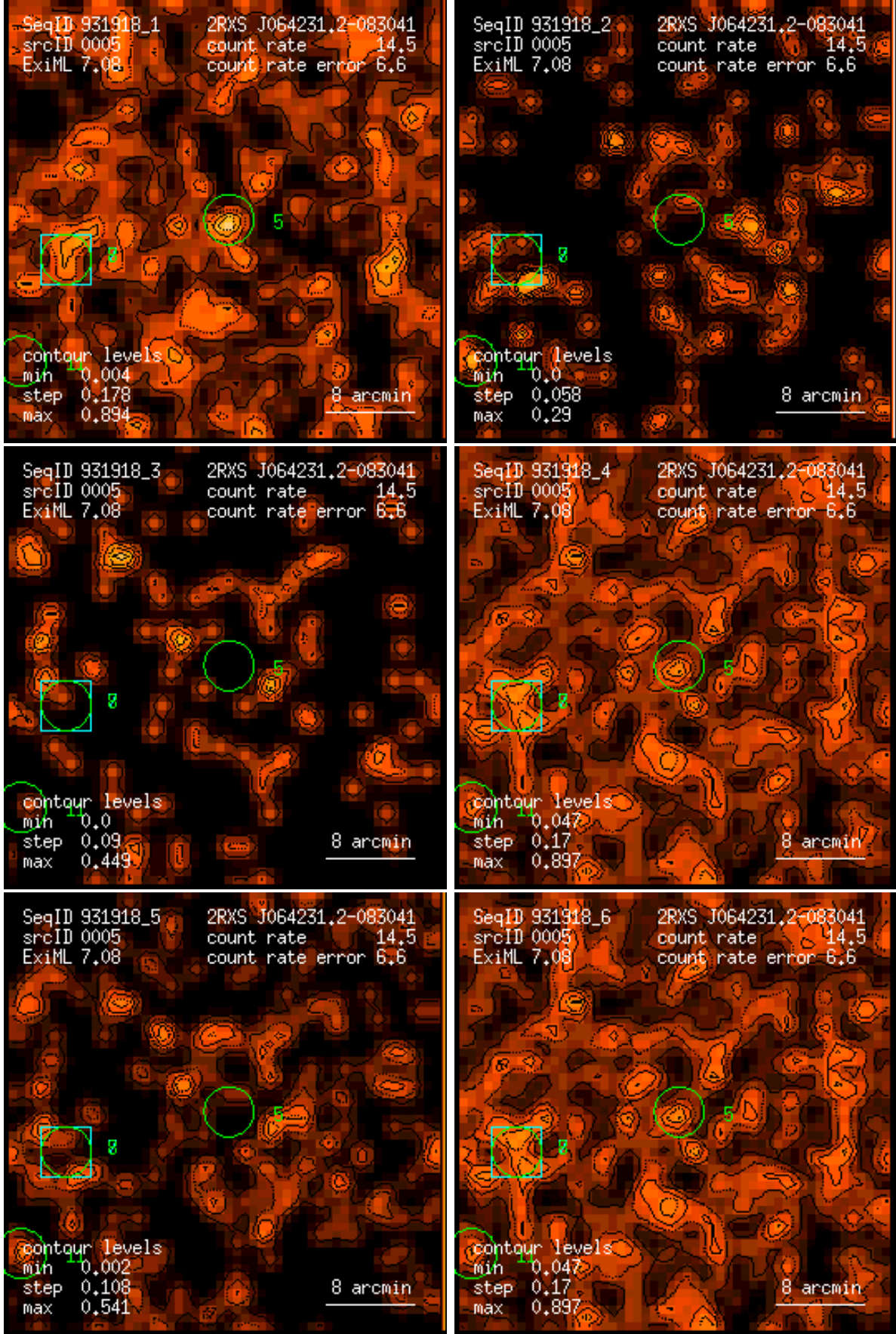
Figure 5: RASS 931918: detection 0005: band rate images, Gaussian filter: (1) PSPC channels 11 – 41, (2) 52 – 90, (3) 91 – 201, (4) 11 – 235, (5) 52 – 201, (6) 11 – 201. Broad band rates in counts/ks. Band rate contour levels in counts/ks/arcmin 2 .
