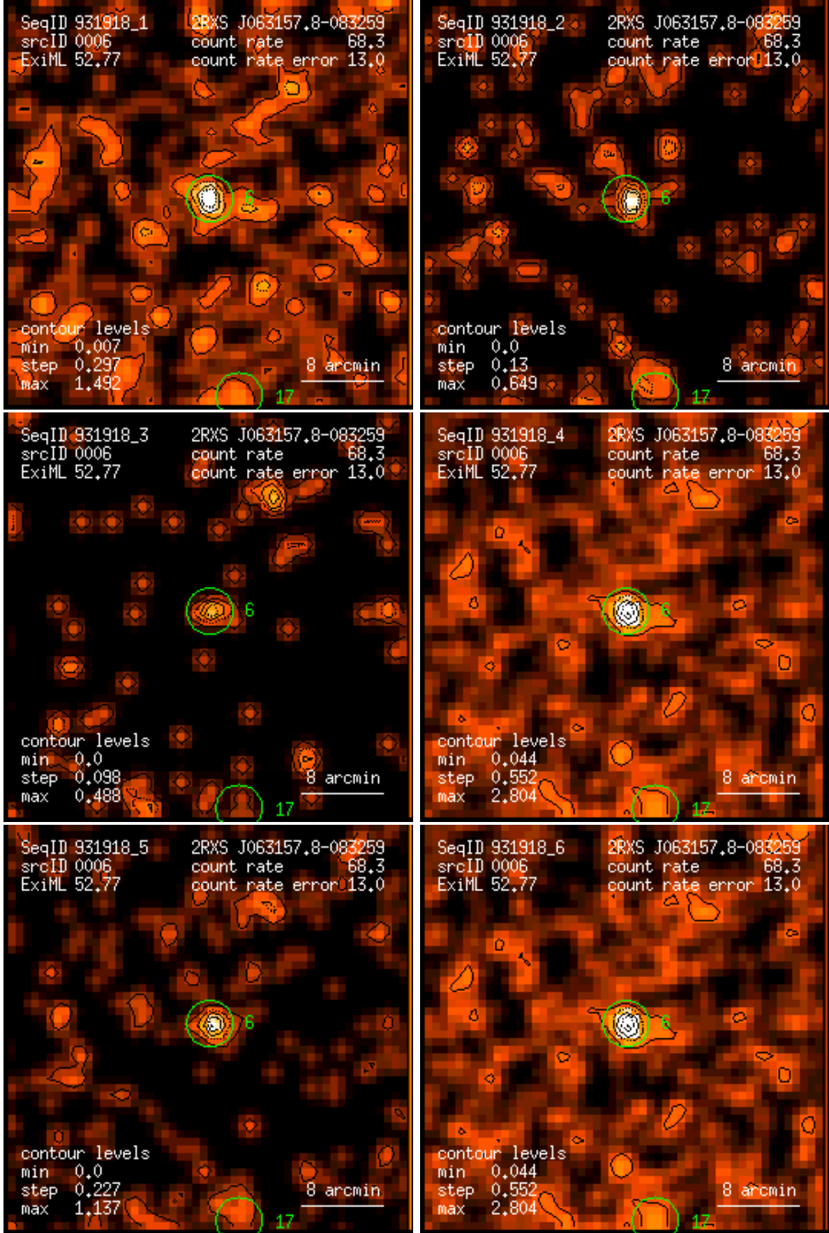
Figure 6: RASS 931918: detection 0006: band rate images, Gaussian filter: (1) PSPC channels 11 – 41, (2) 52 – 90, (3) 91 – 201, (4) 11 – 235, (5) 52 – 201, (6) 11 – 201. Broad band rates in counts/ks. Band rate contour levels in counts/ks/arcmin 2 .
