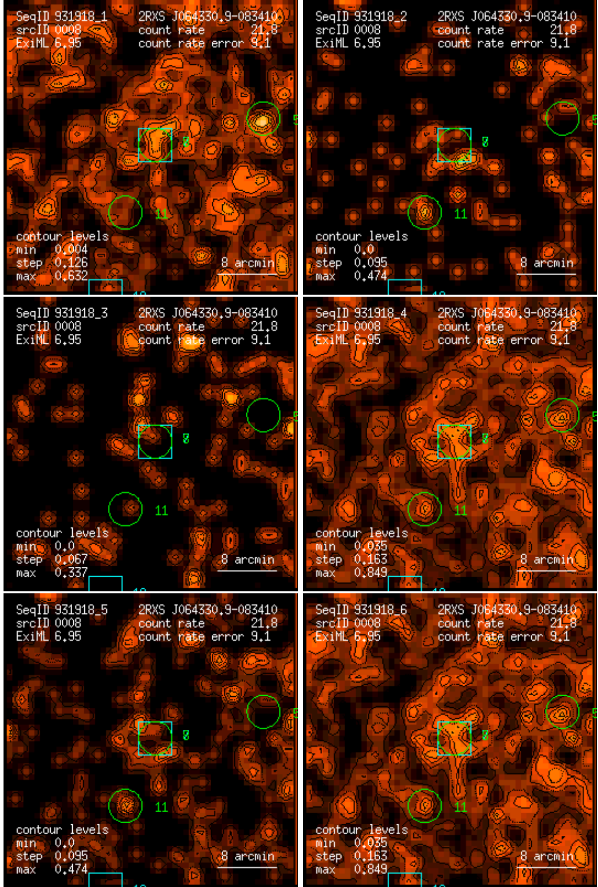
Figure 8: RASS 931918: detection 0008: band rate images, Gaussian filter: (1) PSPC channels 11 – 41, (2) 52 – 90, (3) 91 – 201, (4) 11 – 235, (5) 52 – 201, (6) 11 – 201. Broad band rates in counts/ks. Band rate contour levels in counts/ks/arcmin 2 .
