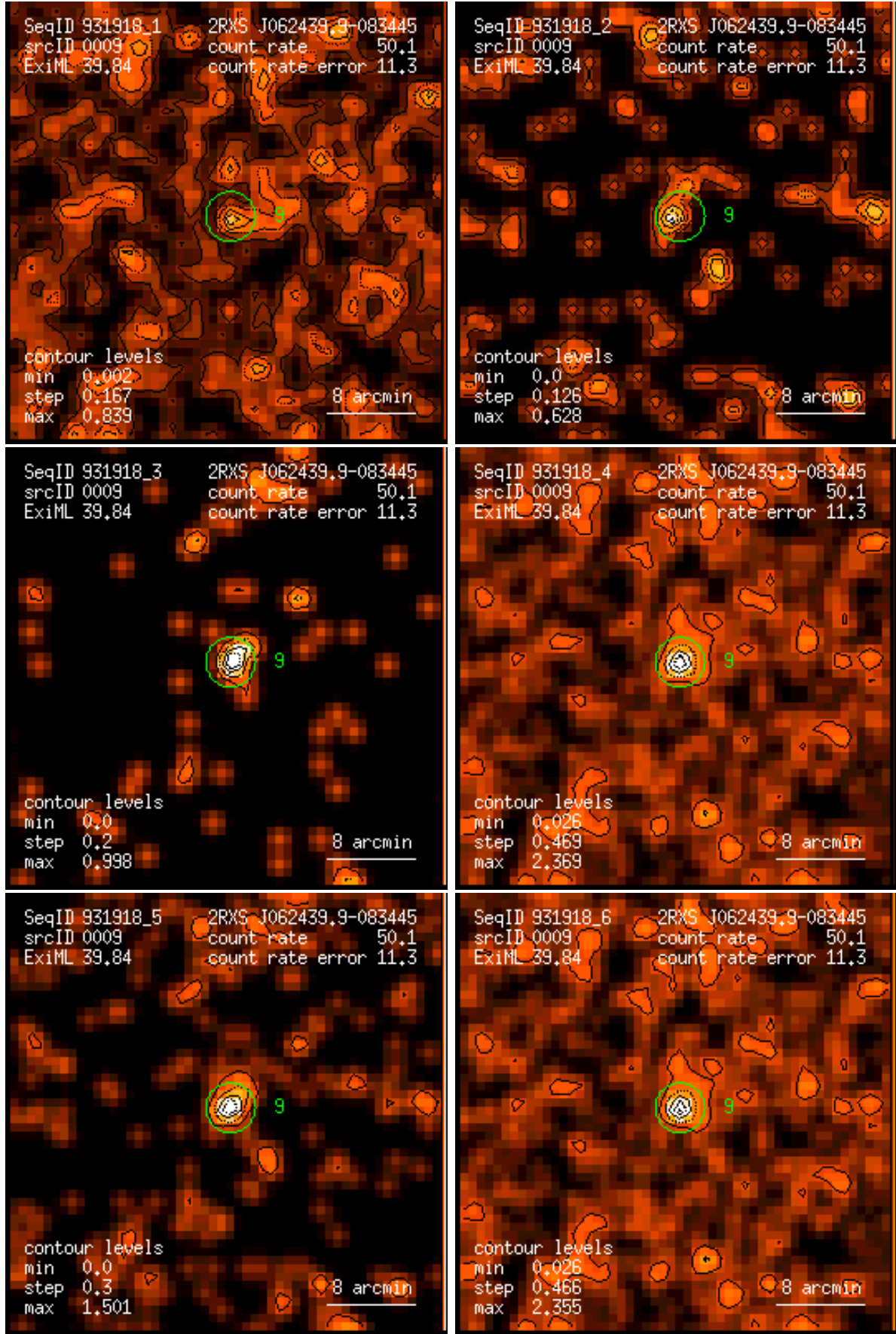
Figure 9: RASS 931918: detection 0009: band rate images, Gaussian filter: (1) PSPC channels 11 – 41, (2) 52 – 90, (3) 91 – 201, (4) 11 – 235, (5) 52 – 201, (6) 11 – 201. Broad band rates in counts/ks. Band rate contour levels in counts/ks/arcmin 2 .
