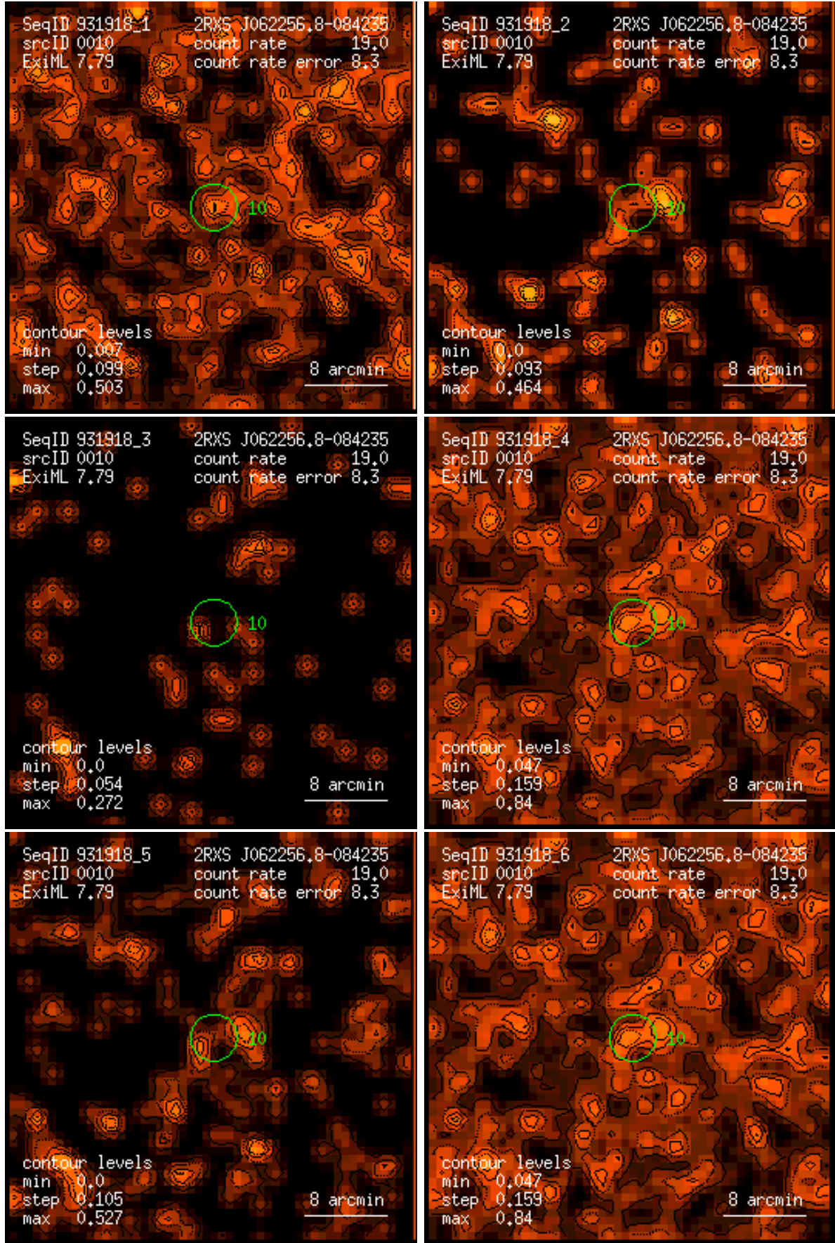
Figure 10: RASS 931918: detection 0010: band rate images, Gaussian filter: (1) PSPC channels 11 – 41, (2) 52 – 90, (3) 91 – 201, (4) 11 – 235, (5) 52 – 201, (6) 11 – 201. Broad band rates in counts/ks. Band rate contour levels in counts/ks/arcmin 2 .
