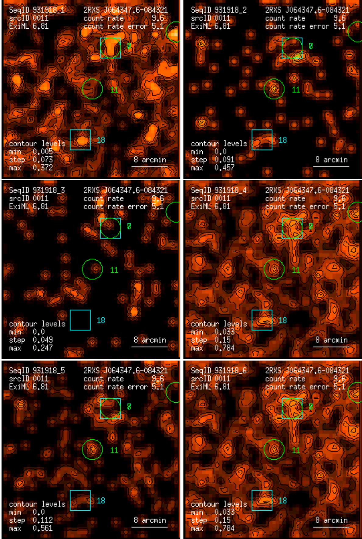
Figure 11: RASS 931918: detection 0011: band rate images, Gaussian filter: (1) PSPC channels 11 – 41, (2) 52 – 90, (3) 91 – 201, (4) 11 – 235, (5) 52 – 201, (6) 11 – 201. Broad band rates in counts/ks. Band rate contour levels in counts/ks/arcmin 2 .
