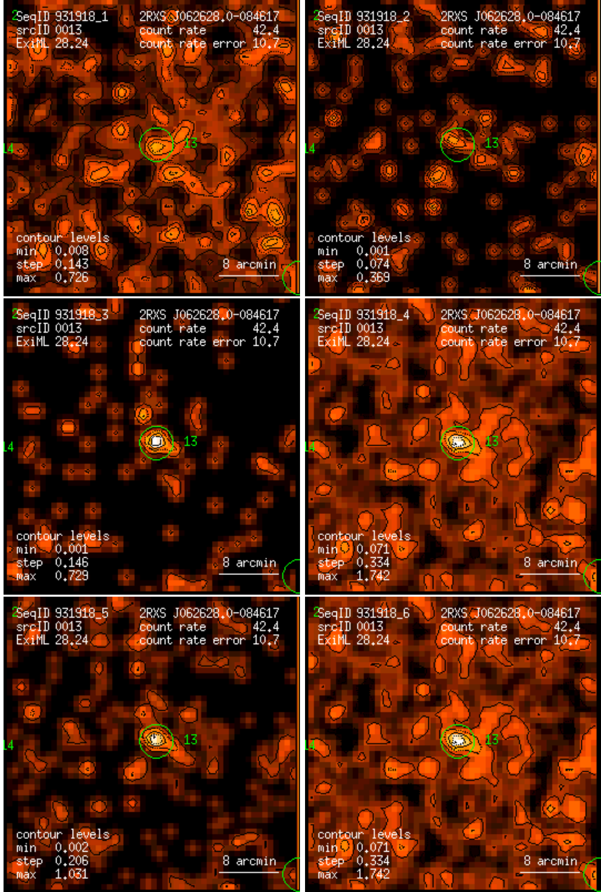
Figure 13: RASS 931918: detection 0013: band rate images, Gaussian filter: (1) PSPC channels 11 – 41, (2) 52 – 90, (3) 91 – 201, (4) 11 – 235, (5) 52 – 201, (6) 11 – 201. Broad band rates in counts/ks. Band rate contour levels in counts/ks/arcmin 2 .
