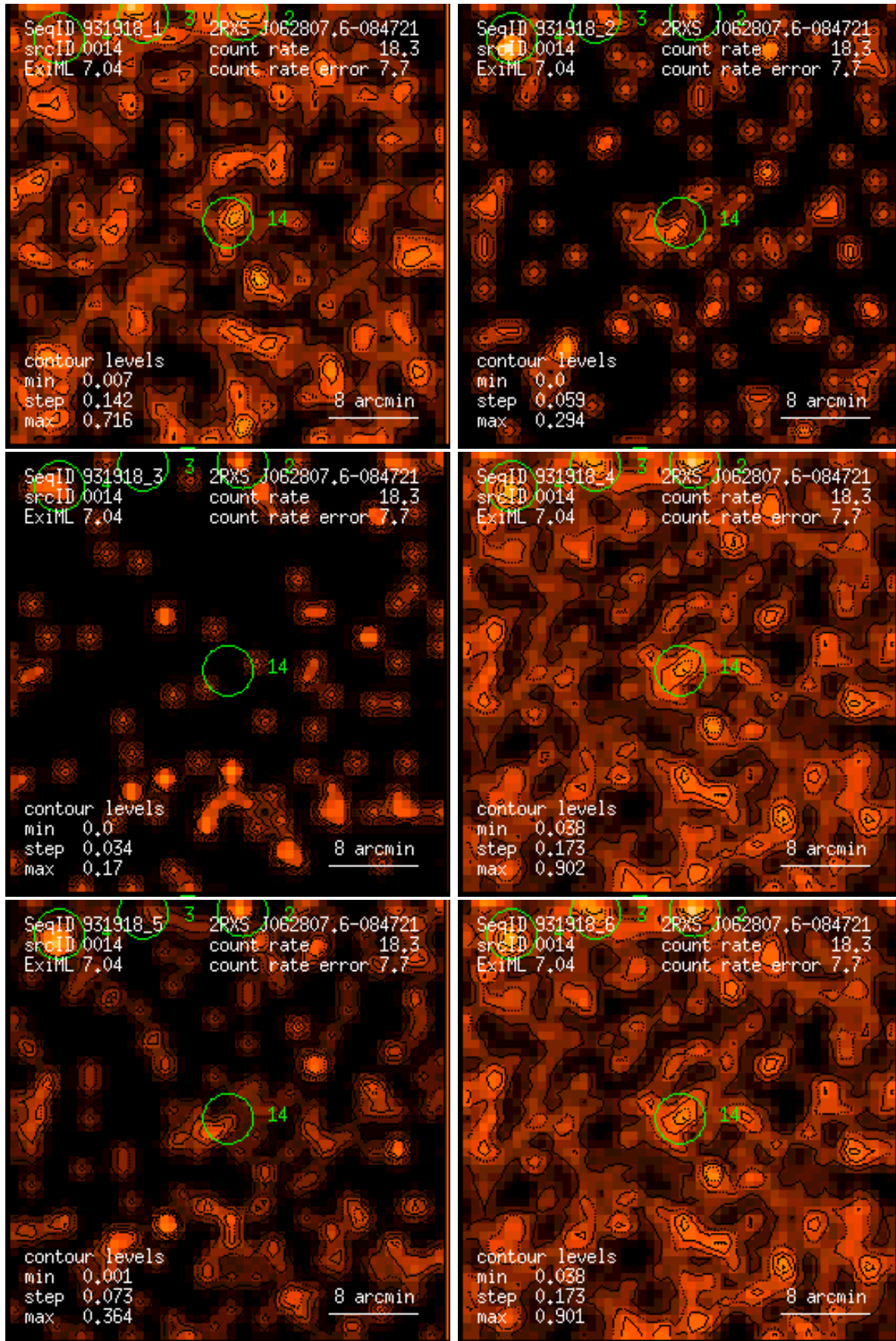
Figure 14: RASS 931918: detection 0014: band rate images, Gaussian filter: (1) PSPC channels 11 – 41, (2) 52 – 90, (3) 91 – 201, (4) 11 – 235, (5) 52 – 201, (6) 11 – 201. Broad band rates in counts/ks. Band rate contour levels in counts/ks/arcmin 2 .
