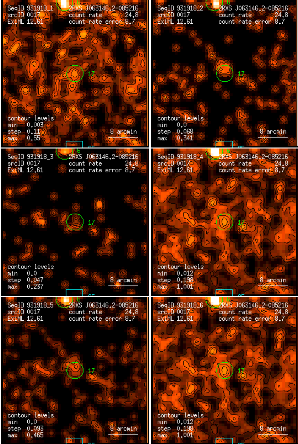
Figure 17: RASS 931918: detection 0017: band rate images, Gaussian filter: (1) PSPC channels 11 – 41, (2) 52 – 90, (3) 91 – 201, (4) 11 – 235, (5) 52 – 201, (6) 11 – 201. Broad band rates in counts/ks. Band rate contour levels in counts/ks/arcmin 2 .
