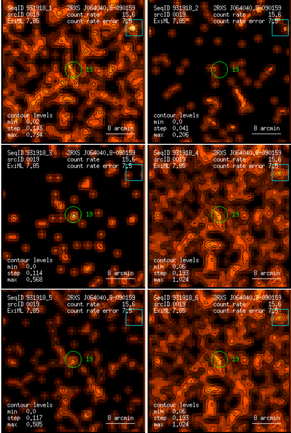
Figure 19: RASS 931918: detection 0019: band rate images, Gaussian filter: (1) PSPC channels 11 – 41, (2) 52 – 90, (3) 91 – 201, (4) 11 – 235, (5) 52 – 201, (6) 11 – 201. Broad band rates in counts/ks. Band rate contour levels in counts/ks/arcmin 2 .
