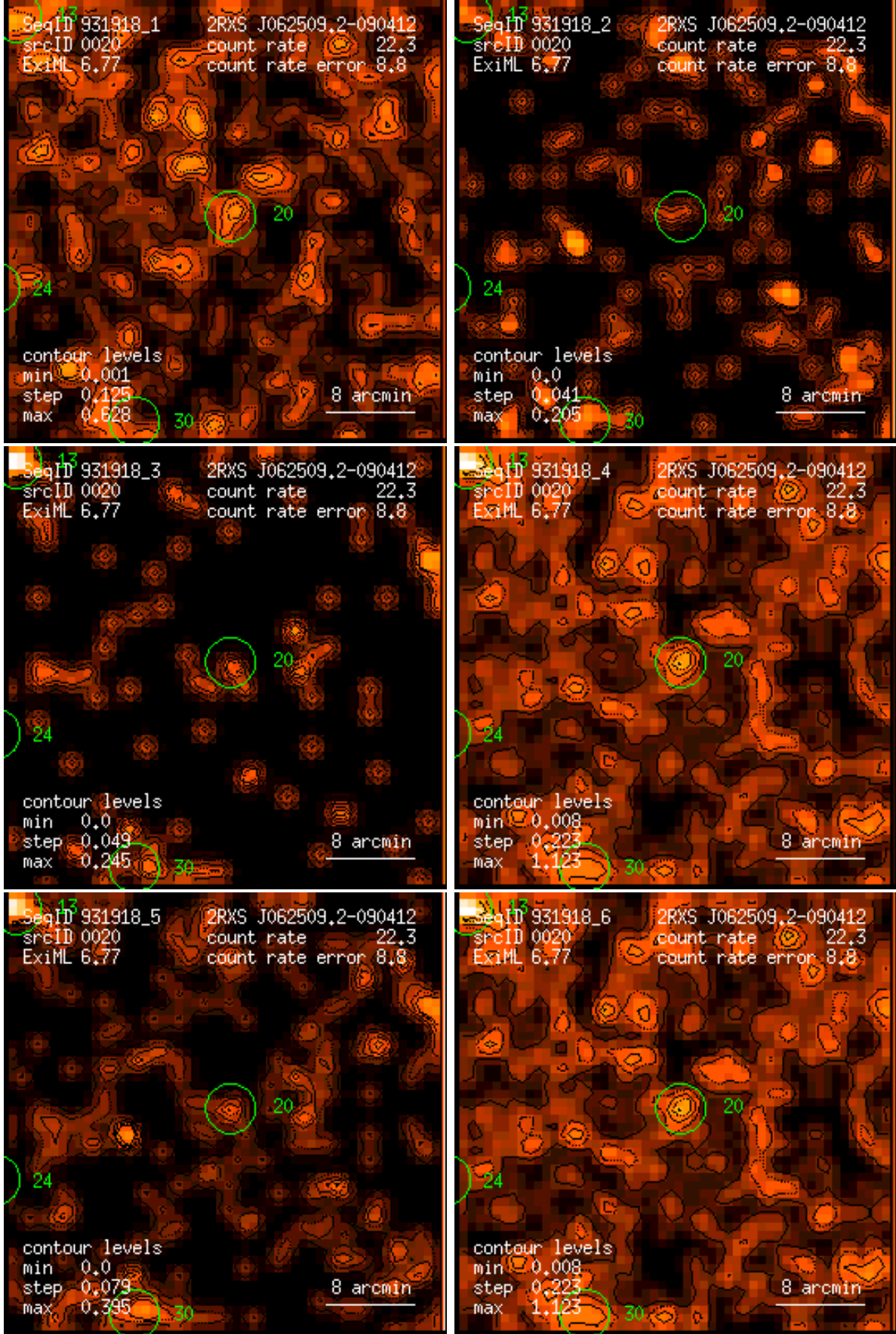
Figure 20: RASS 931918: detection 0020: band rate images, Gaussian filter: (1) PSPC channels 11 – 41, (2) 52 – 90, (3) 91 – 201, (4) 11 – 235, (5) 52 – 201, (6) 11 – 201. Broad band rates in counts/ks. Band rate contour levels in counts/ks/arcmin 2 .
