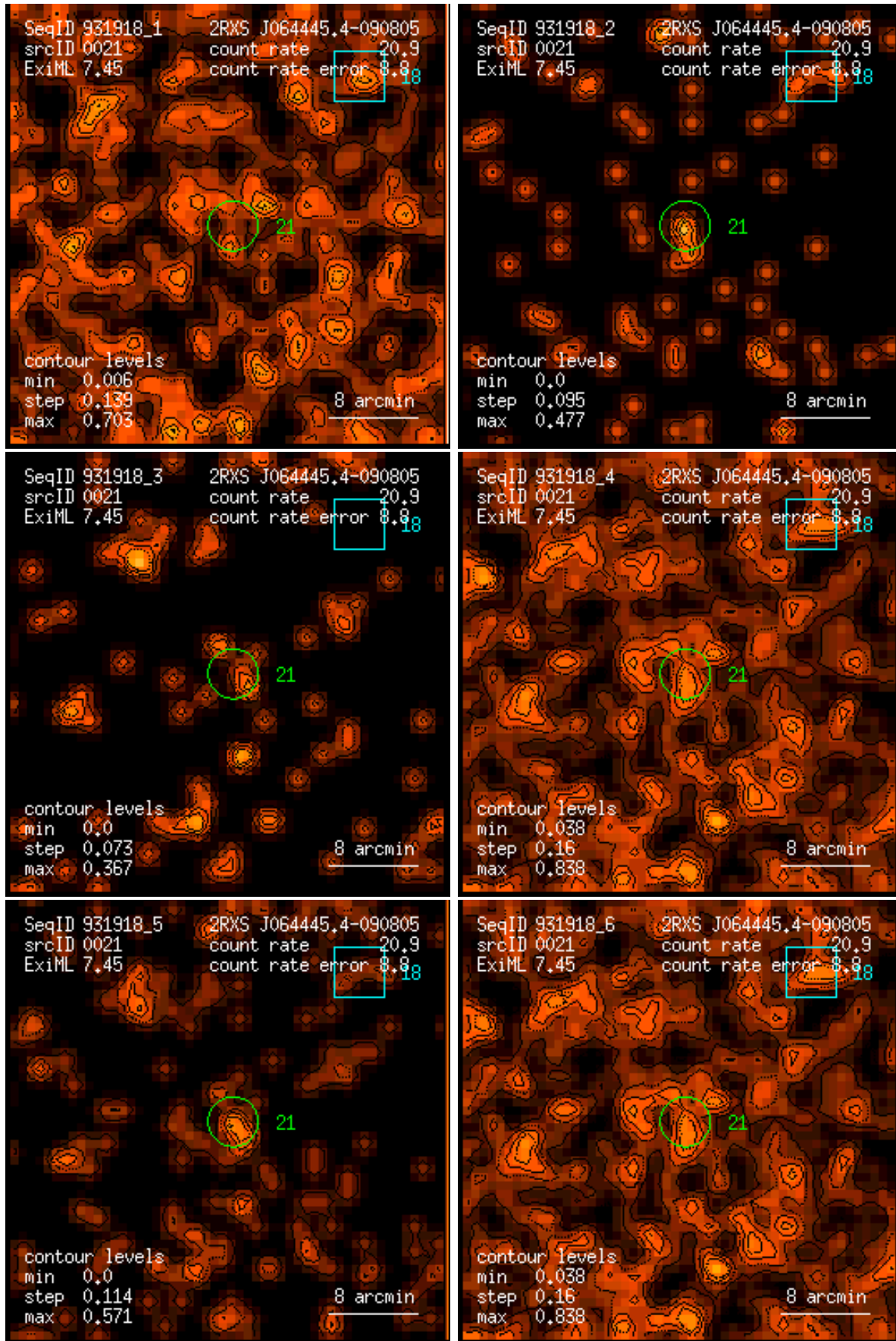
Figure 21: RASS 931918: detection 0021: band rate images, Gaussian filter: (1) PSPC channels 11 – 41, (2) 52 – 90, (3) 91 – 201, (4) 11 – 235, (5) 52 – 201, (6) 11 – 201. Broad band rates in counts/ks. Band rate contour levels in counts/ks/arcmin 2 .
