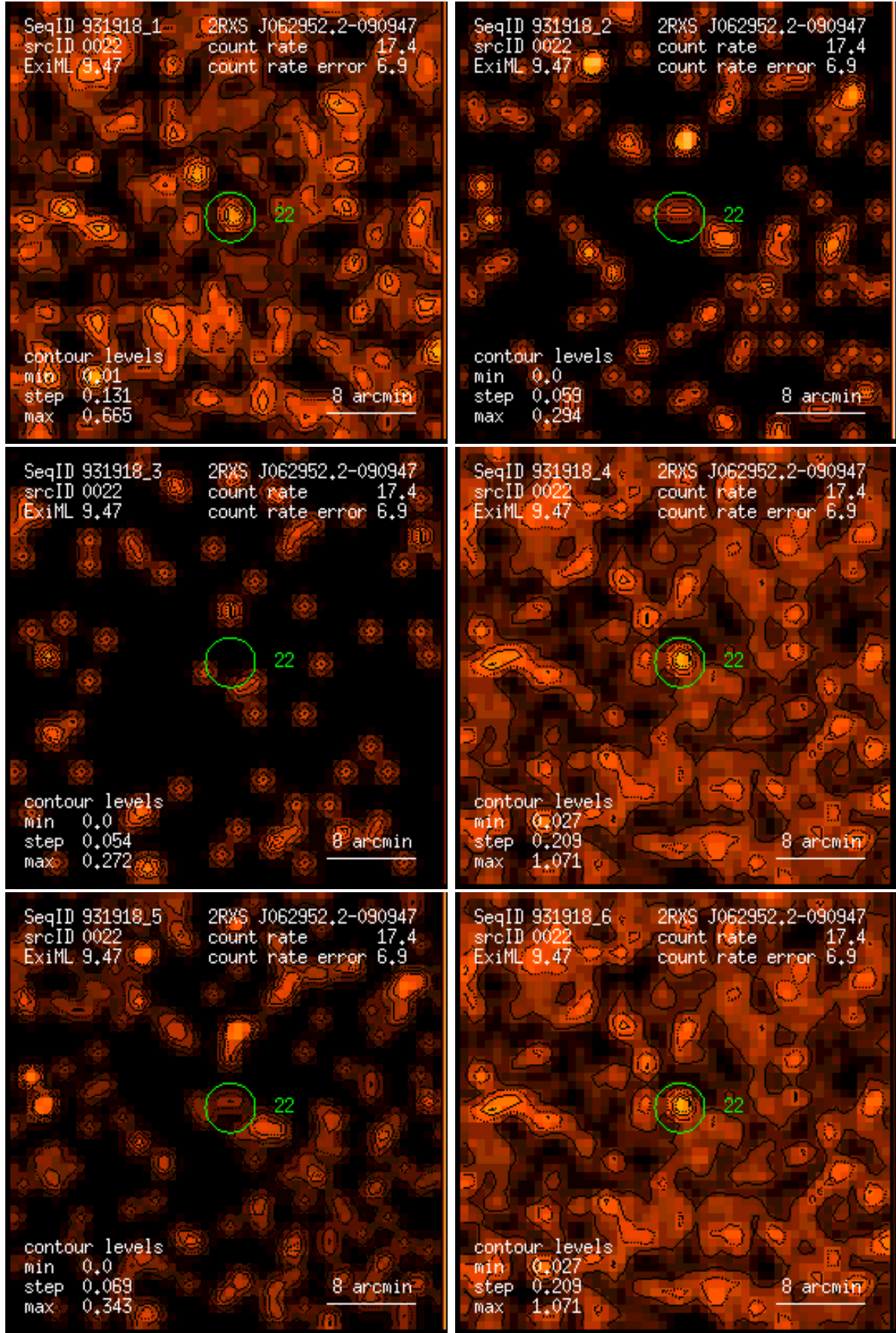
Figure 22: RASS 931918: detection 0022: band rate images, Gaussian filter: (1) PSPC channels 11 – 41, (2) 52 – 90, (3) 91 – 201, (4) 11 – 235, (5) 52 – 201, (6) 11 – 201. Broad band rates in counts/ks. Band rate contour levels in counts/ks/arcmin 2 .
