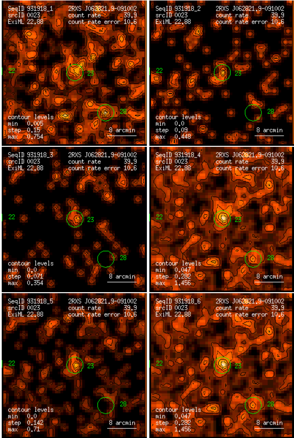
Figure 23: RASS 931918: detection 0023: band rate images, Gaussian filter: (1) PSPC channels 11 – 41, (2) 52 – 90, (3) 91 – 201, (4) 11 – 235, (5) 52 – 201, (6) 11 – 201. Broad band rates in counts/ks. Band rate contour levels in counts/ks/arcmin 2 .
