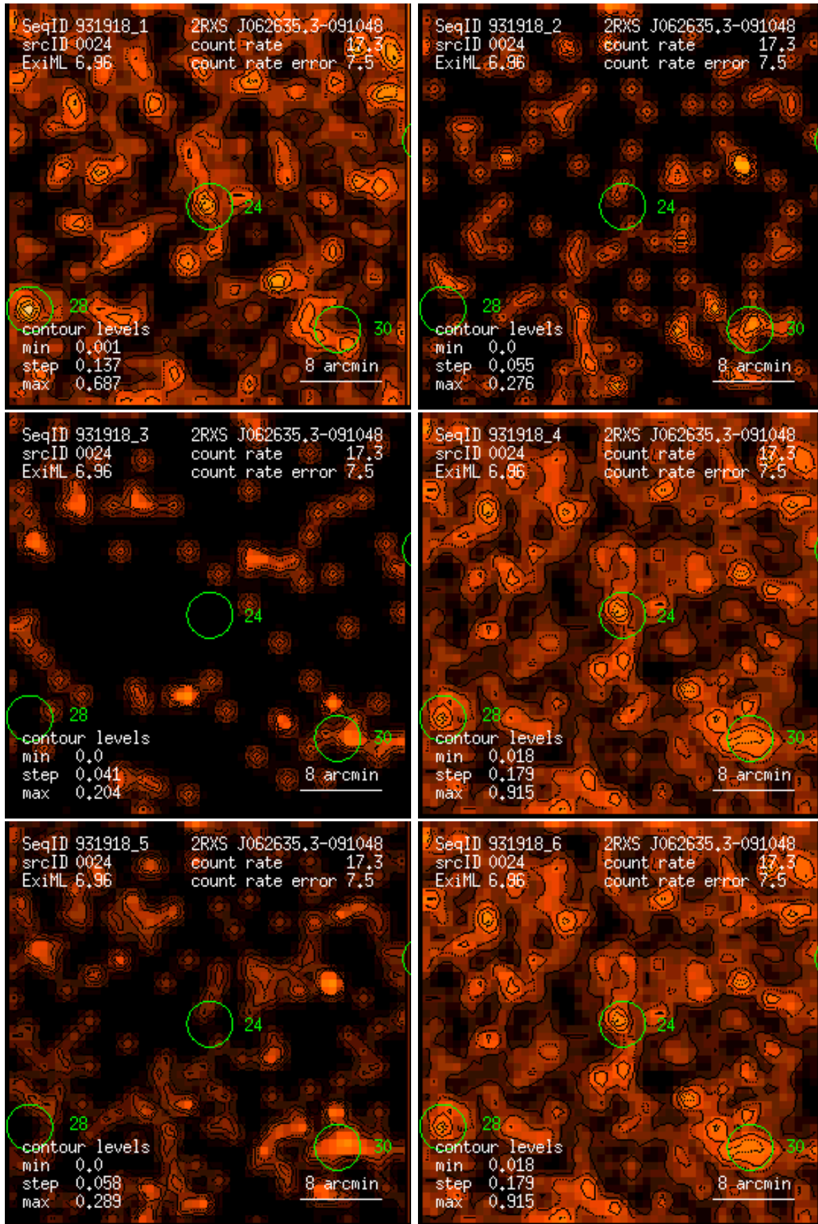
Figure 24: RASS 931918: detection 0024: band rate images, Gaussian filter: (1) PSPC channels 11 – 41, (2) 52 – 90, (3) 91 – 201, (4) 11 – 235, (5) 52 – 201, (6) 11 – 201. Broad band rates in counts/ks. Band rate contour levels in counts/ks/arcmin 2 .
