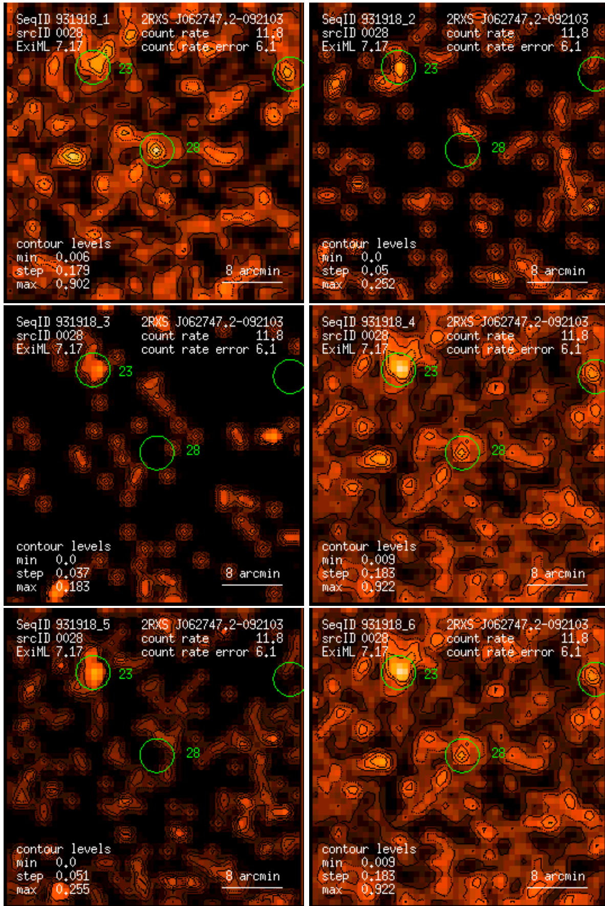
Figure 28: RASS 931918: detection 0028: band rate images, Gaussian filter: (1) PSPC channels 11 – 41, (2) 52 – 90, (3) 91 – 201, (4) 11 – 235, (5) 52 – 201, (6) 11 – 201. Broad band rates in counts/ks. Band rate contour levels in counts/ks/arcmin 2 .
