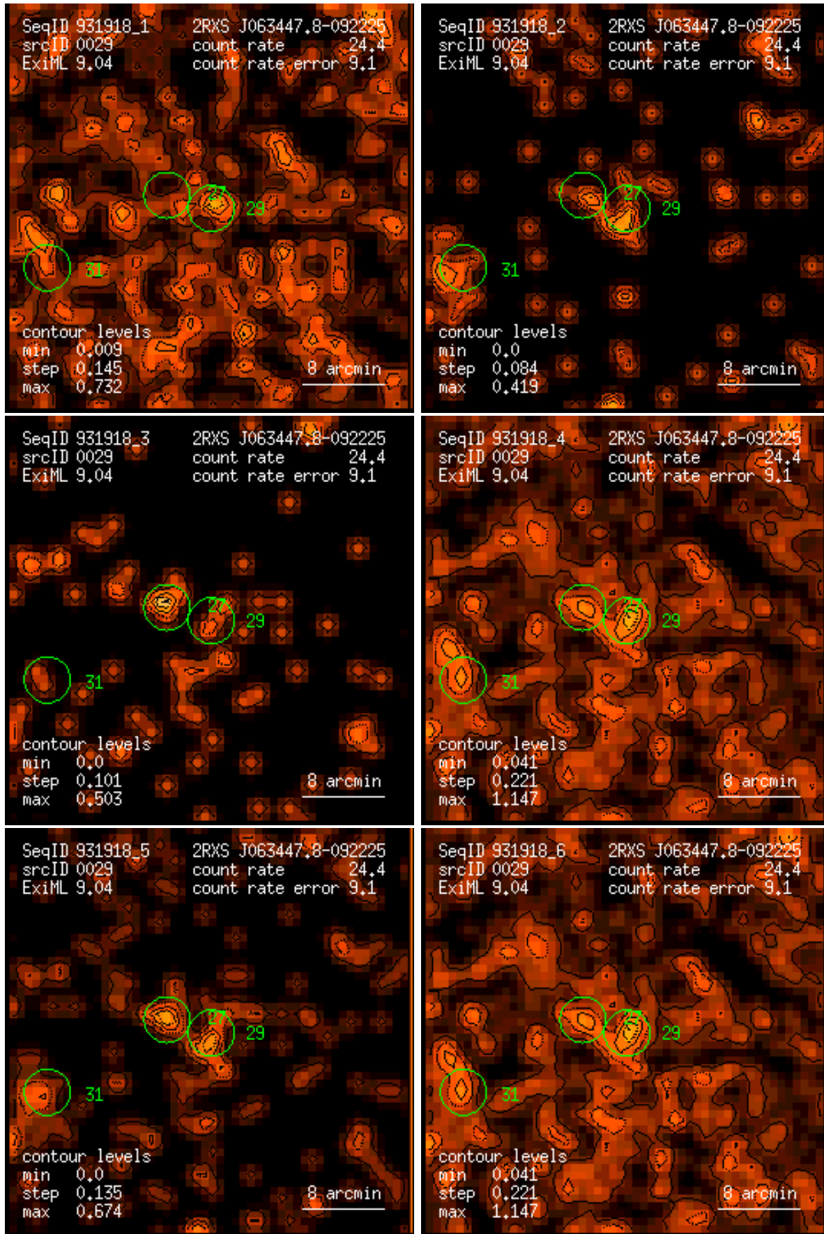
Figure 29: RASS 931918: detection 0029: band rate images, Gaussian filter: (1) PSPC channels 11 – 41, (2) 52 – 90, (3) 91 – 201, (4) 11 – 235, (5) 52 – 201, (6) 11 – 201. Broad band rates in counts/ks. Band rate contour levels in counts/ks/arcmin 2 .
