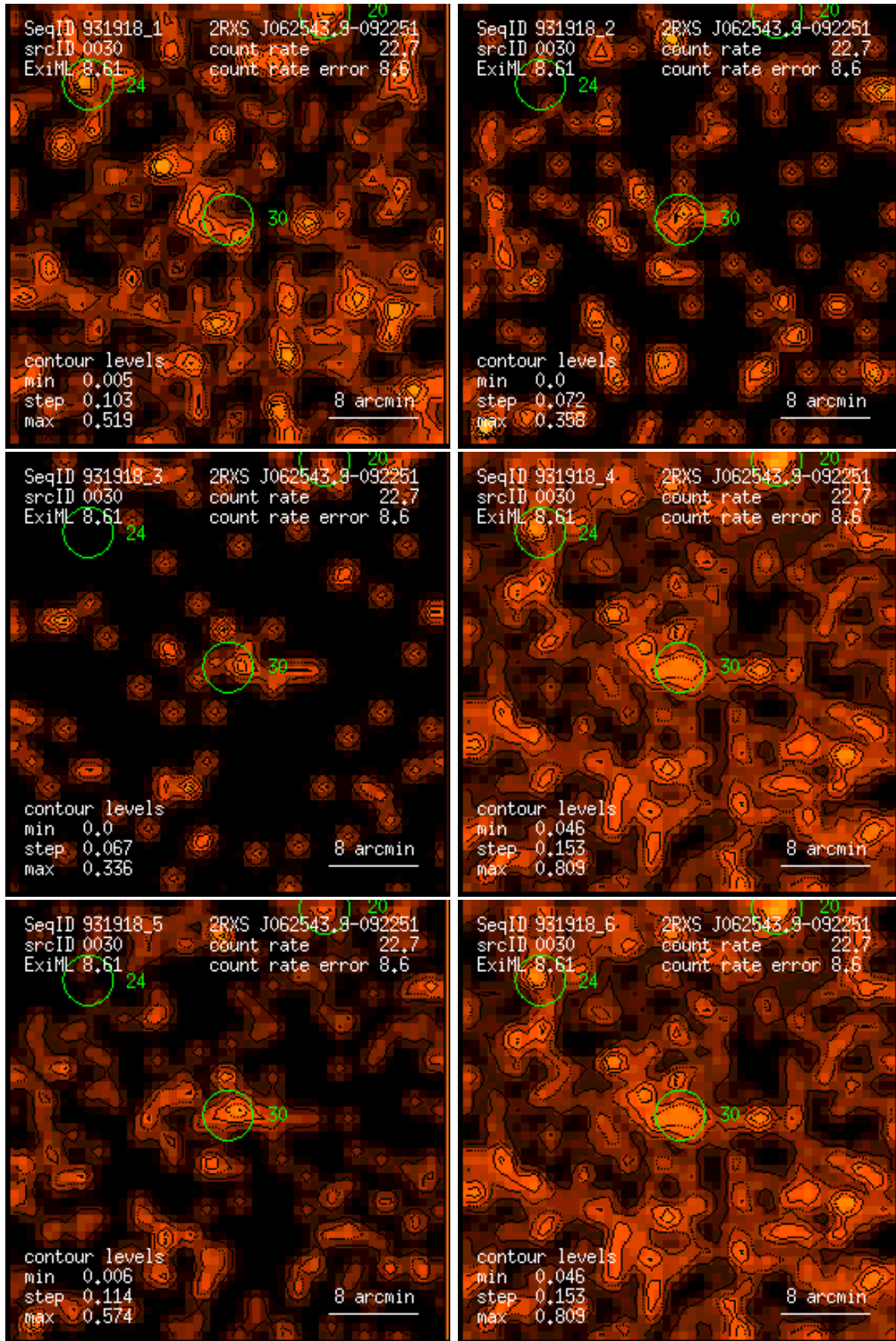
Figure 30: RASS 931918: detection 0030: band rate images, Gaussian filter: (1) PSPC channels 11 – 41, (2) 52 – 90, (3) 91 – 201, (4) 11 – 235, (5) 52 – 201, (6) 11 – 201. Broad band rates in counts/ks. Band rate contour levels in counts/ks/arcmin 2 .
