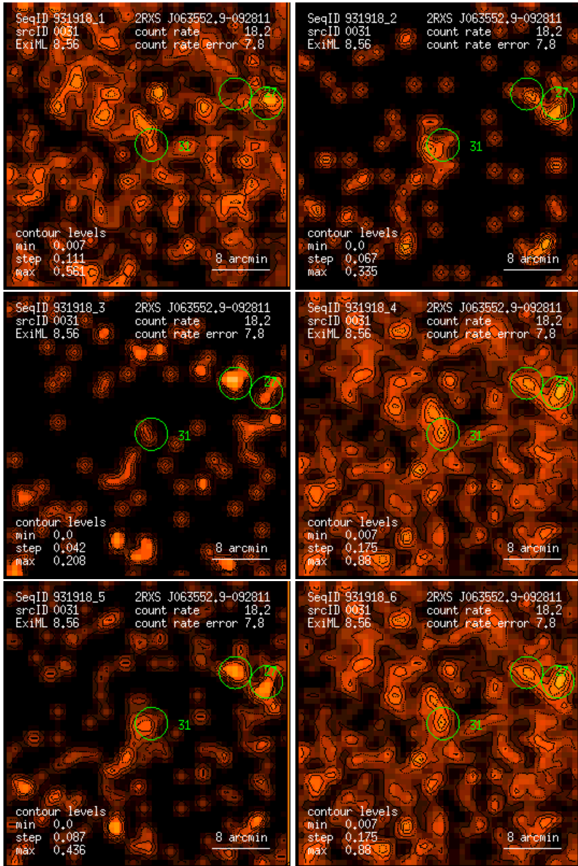
Figure 31: RASS 931918: detection 0031: band rate images, Gaussian filter: (1) PSPC channels 11 – 41, (2) 52 – 90, (3) 91 – 201, (4) 11 – 235, (5) 52 – 201, (6) 11 – 201. Broad band rates in counts/ks. Band rate contour levels in counts/ks/arcmin 2 .
