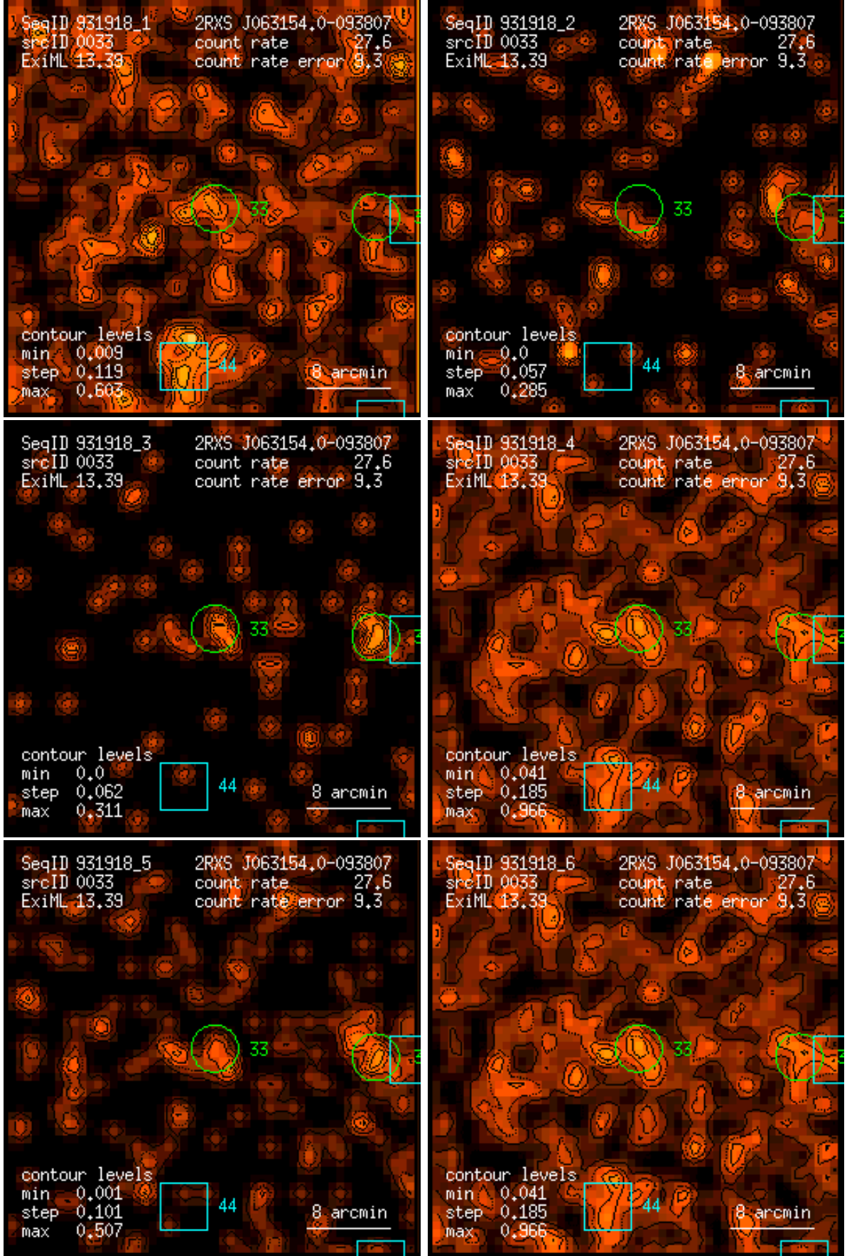
Figure 33: RASS 931918: detection 0033: band rate images, Gaussian filter: (1) PSPC channels 11 – 41, (2) 52 – 90, (3) 91 – 201, (4) 11 – 235, (5) 52 – 201, (6) 11 – 201. Broad band rates in counts/ks. Band rate contour levels in counts/ks/arcmin 2 .
