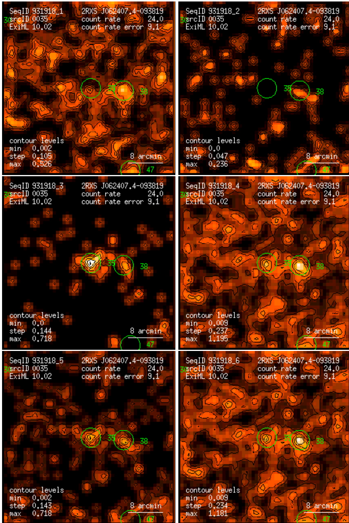
Figure 35: RASS 931918: detection 0035: band rate images, Gaussian filter: (1) PSPC channels 11 – 41, (2) 52 – 90, (3) 91 – 201, (4) 11 – 235, (5) 52 – 201, (6) 11 – 201. Broad band rates in counts/ks. Band rate contour levels in counts/ks/arcmin 2 .
