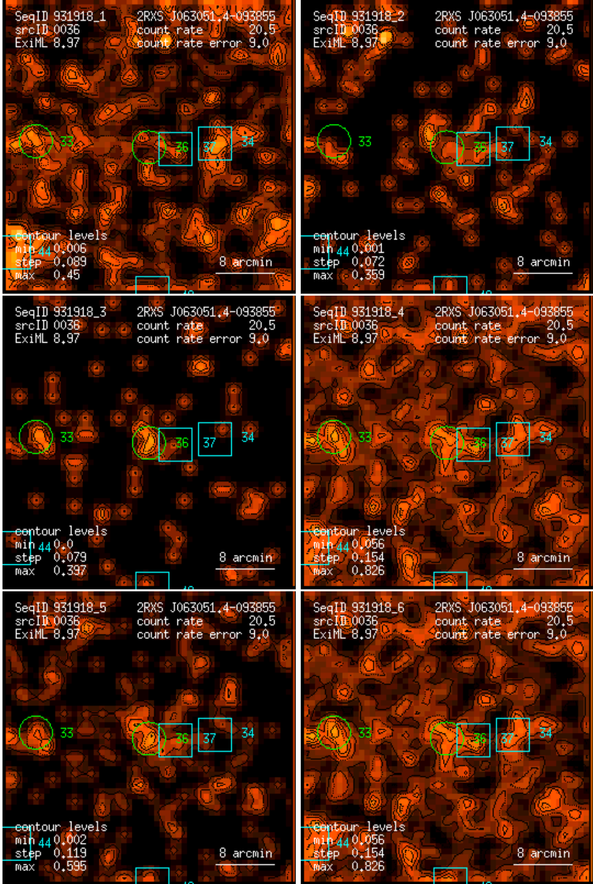
Figure 36: RASS 931918: detection 0036: band rate images, Gaussian filter: (1) PSPC channels 11 – 41, (2) 52 – 90, (3) 91 – 201, (4) 11 – 235, (5) 52 – 201, (6) 11 – 201. Broad band rates in counts/ks. Band rate contour levels in counts/ks/arcmin 2 .
