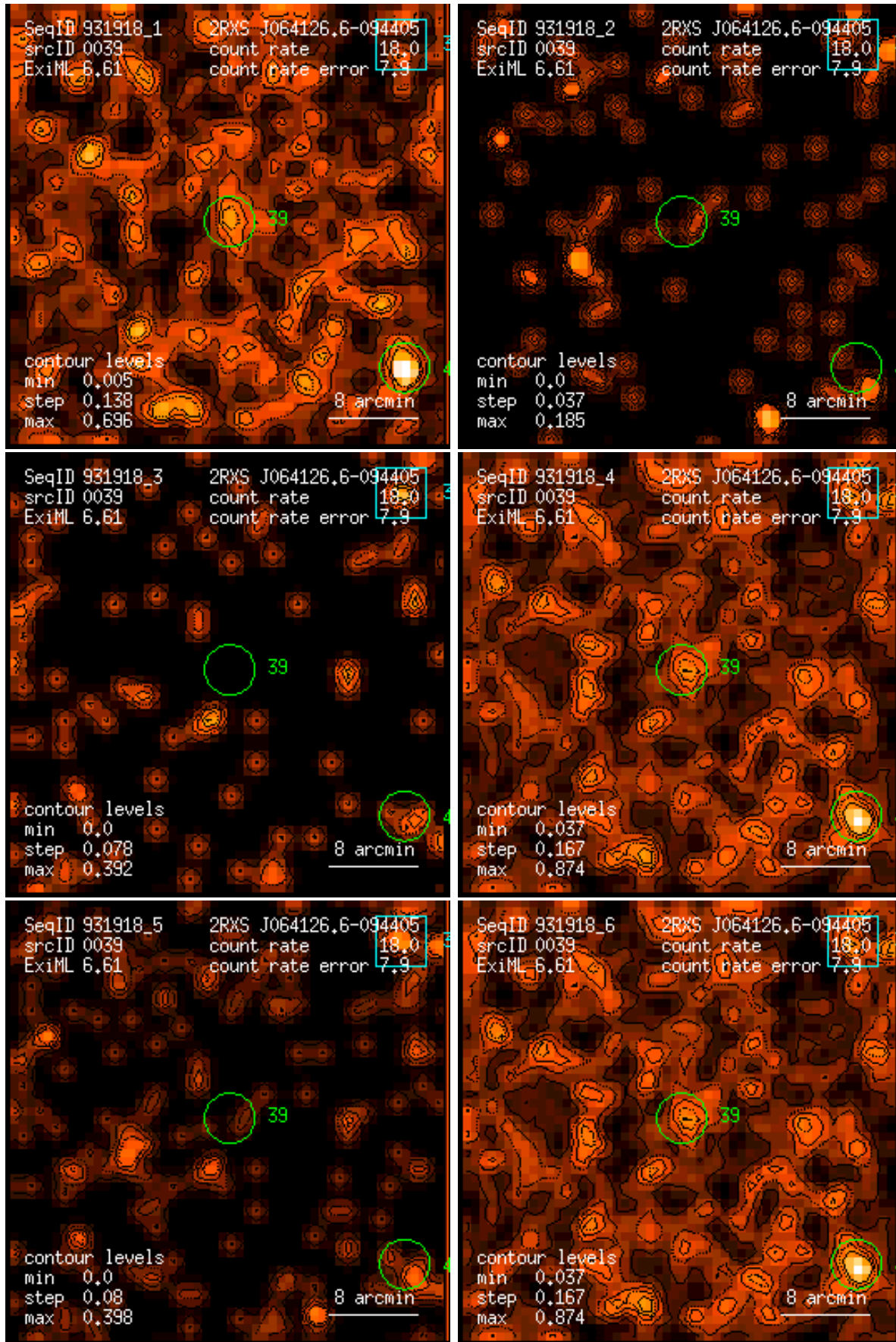
Figure 39: RASS 931918: detection 0039: band rate images, Gaussian filter: (1) PSPC channels 11 – 41, (2) 52 – 90, (3) 91 – 201, (4) 11 – 235, (5) 52 – 201, (6) 11 – 201. Broad band rates in counts/ks. Band rate contour levels in counts/ks/arcmin 2 .
