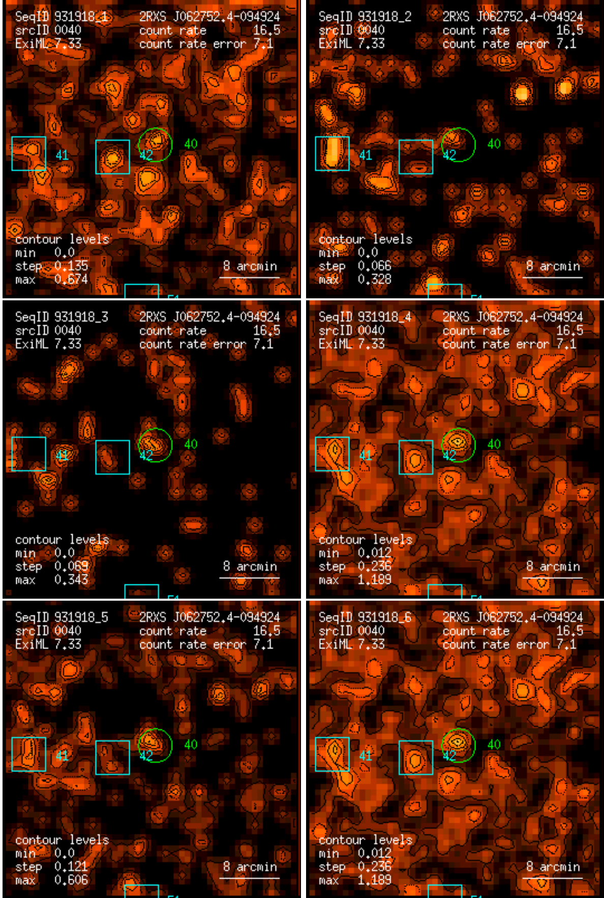
Figure 40: RASS 931918: detection 0040: band rate images, Gaussian filter: (1) PSPC channels 11 – 41, (2) 52 – 90, (3) 91 – 201, (4) 11 – 235, (5) 52 – 201, (6) 11 – 201. Broad band rates in counts/ks. Band rate contour levels in counts/ks/arcmin 2 .
