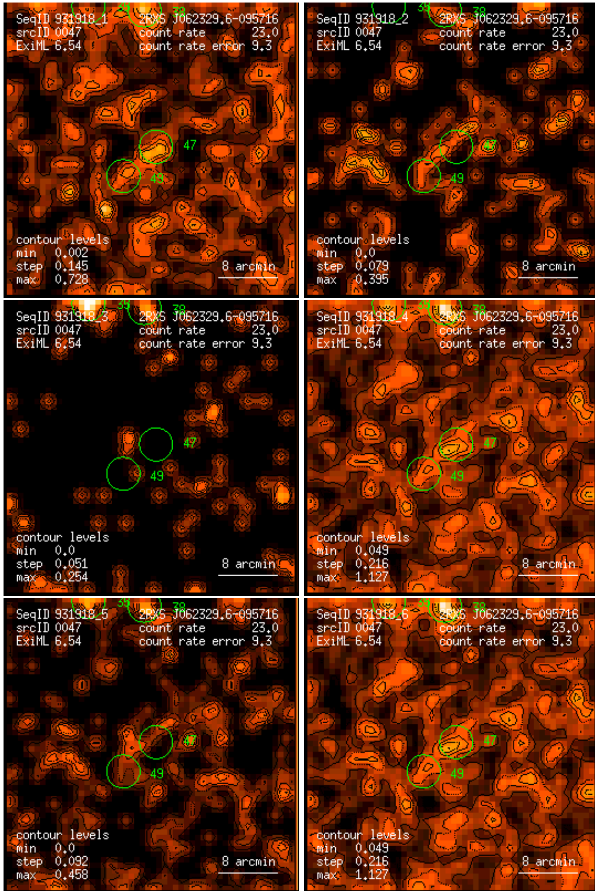
Figure 47: RASS 931918: detection 0047: band rate images, Gaussian filter: (1) PSPC channels 11 – 41, (2) 52 – 90, (3) 91 – 201, (4) 11 – 235, (5) 52 – 201, (6) 11 – 201. Broad band rates in counts/ks. Band rate contour levels in counts/ks/arcmin 2 .
