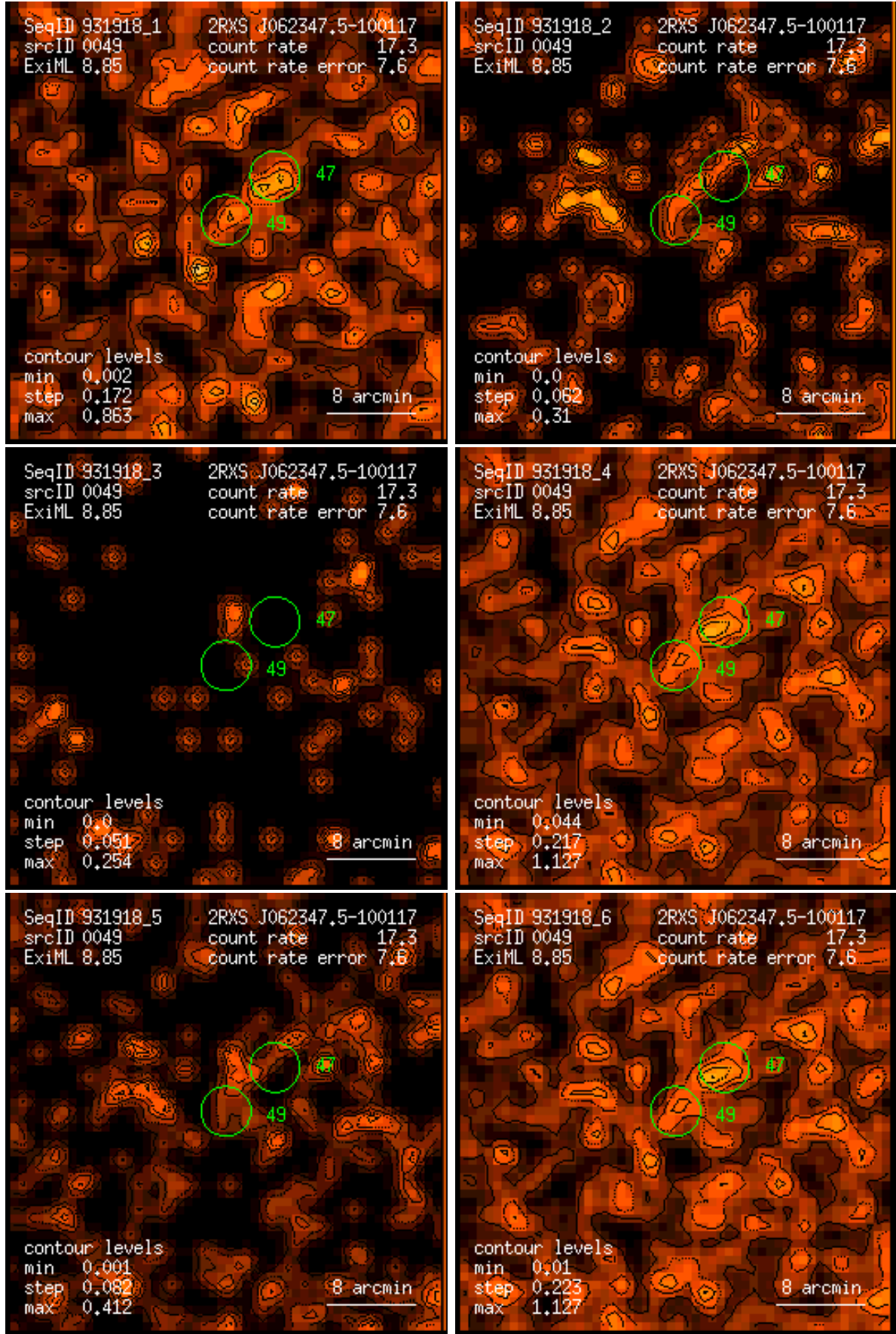
Figure 49: RASS 931918: detection 0049: band rate images, Gaussian filter: (1) PSPC channels 11 – 41, (2) 52 – 90, (3) 91 – 201, (4) 11 – 235, (5) 52 – 201, (6) 11 – 201. Broad band rates in counts/ks. Band rate contour levels in counts/ks/arcmin 2 .
